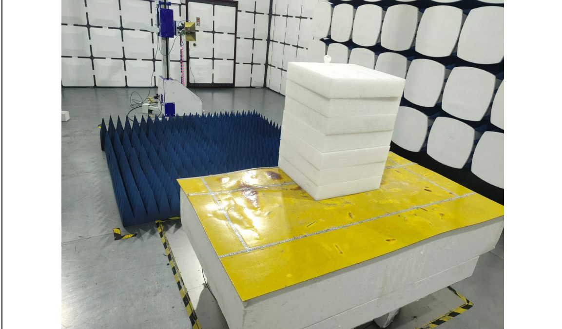
Emissions in frequency bands (above 1GHz)
