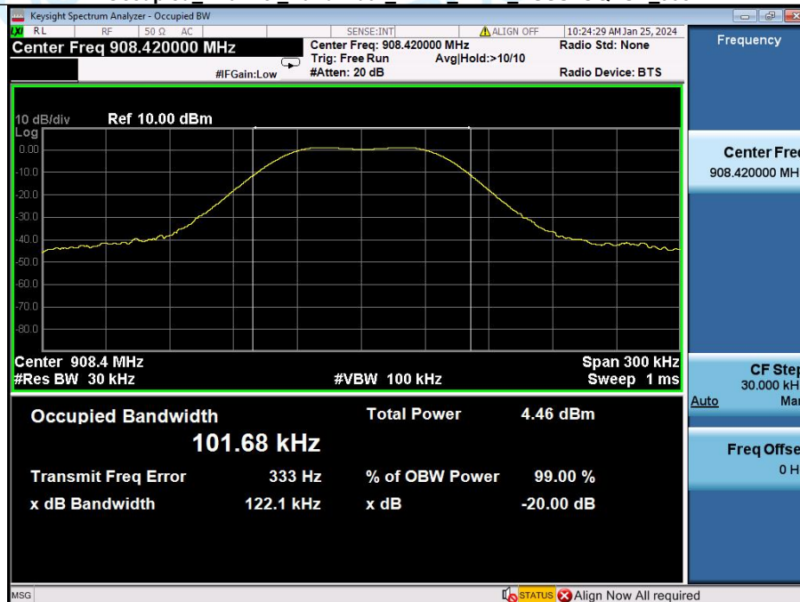
Occupied_Channel_Bandwidth_NVNT_ANT1_DSSS/OQPSK_908.42
