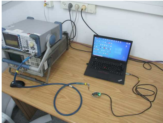
Figure 1. Conducted Emission Test
