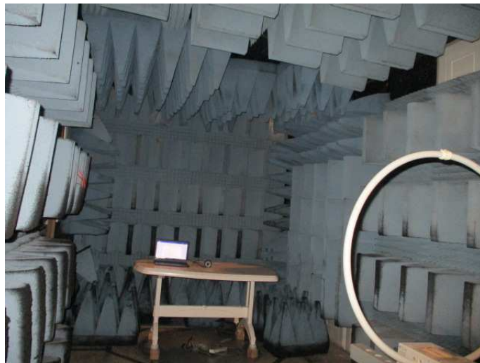
Figure 2. Radiated Emission Test, 0.009-30MHz
