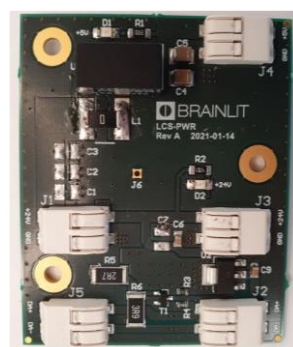
LCS PWR Board – 24/5V power to the LCS board
