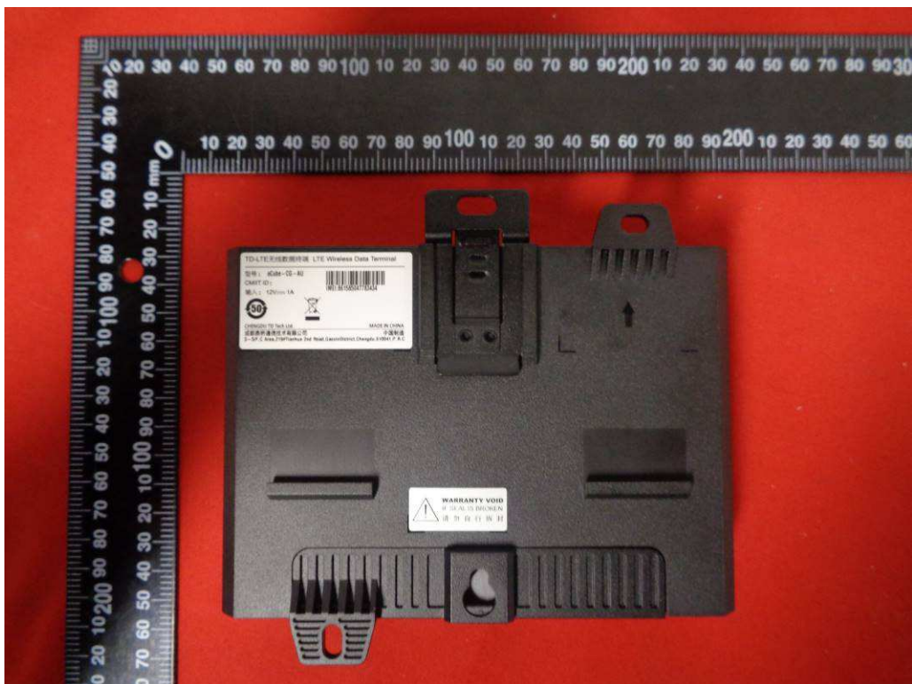
Pic.8 eCube-CG-AU bottom view
