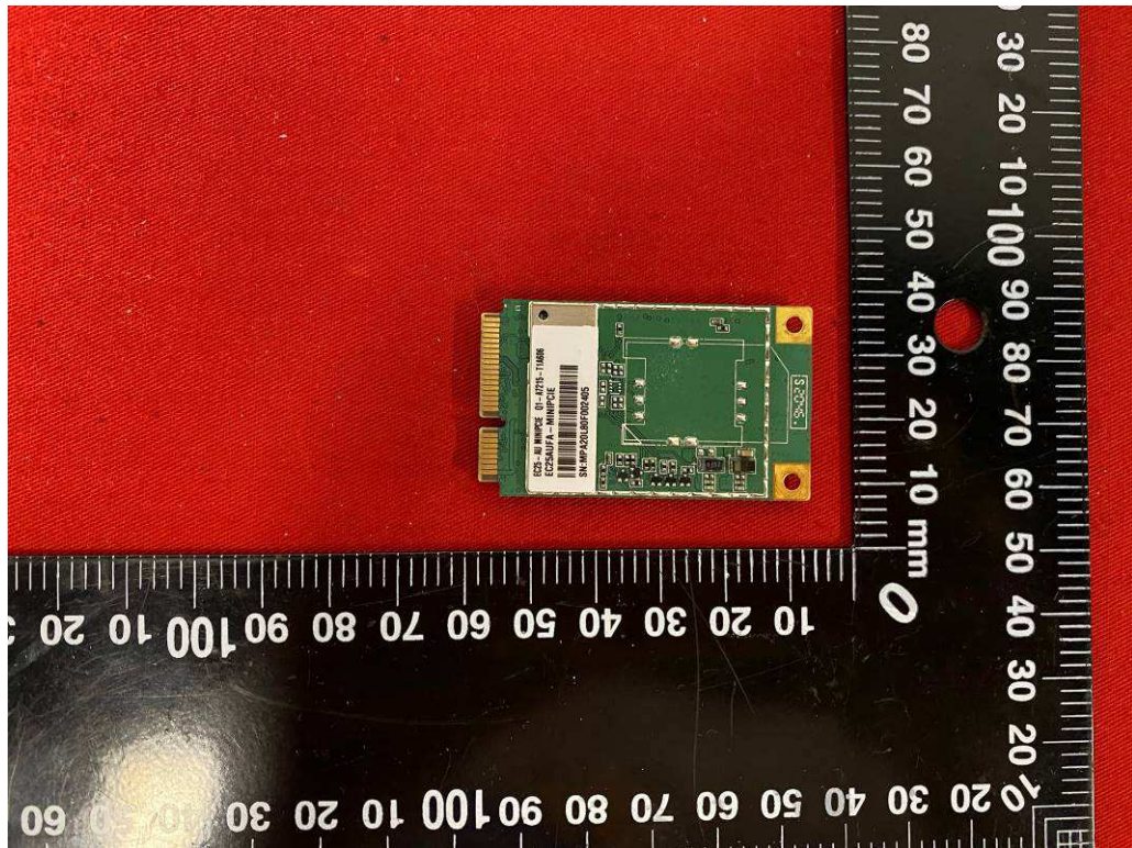
Pic.7 eCube-CP-AU bottom view of EC25-AU
