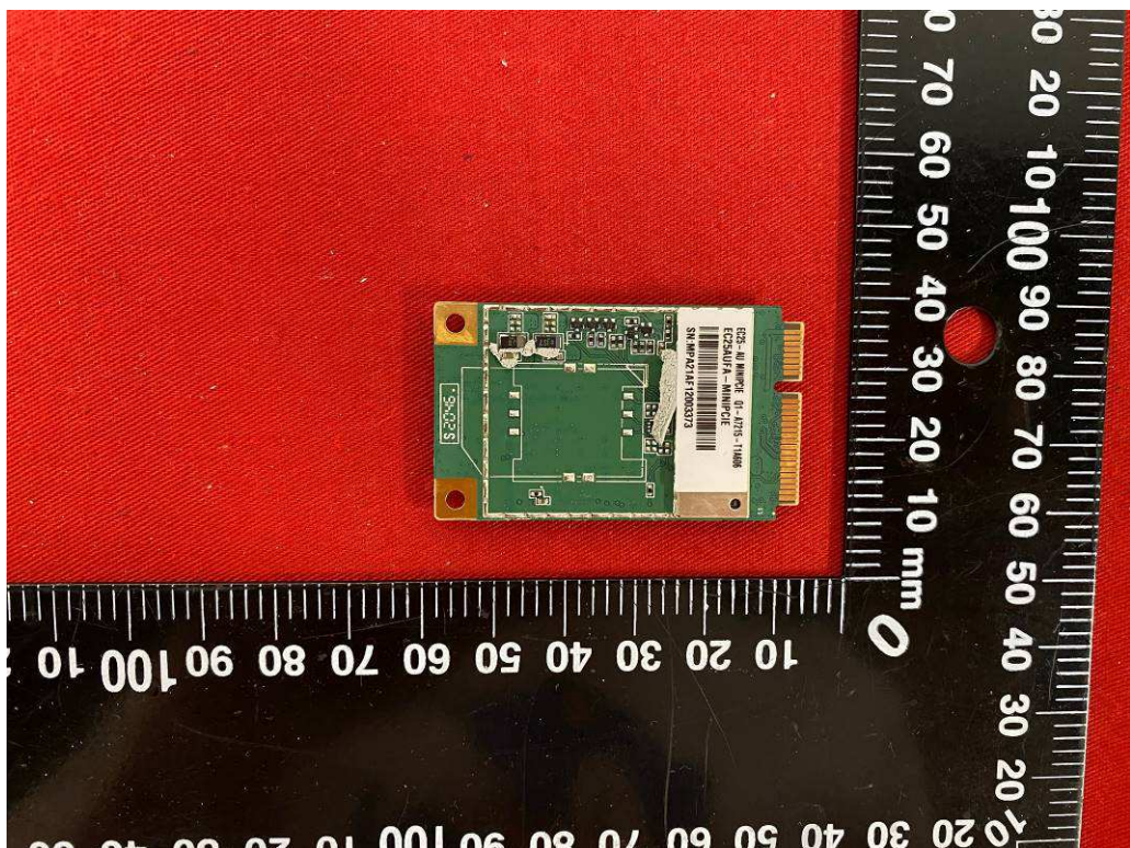
Pic.14 eCube-CG-AU bottom view of PCB EC25-AU
