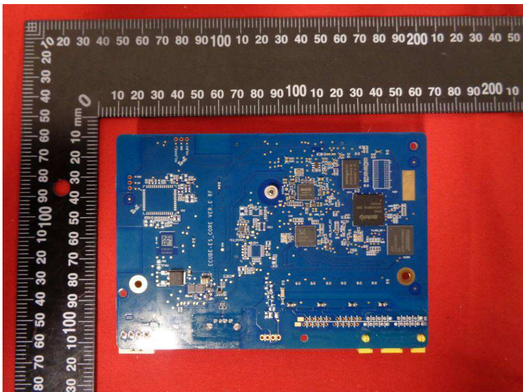
Pic.12 eCube-CG-AU bottom view of PCB 2
