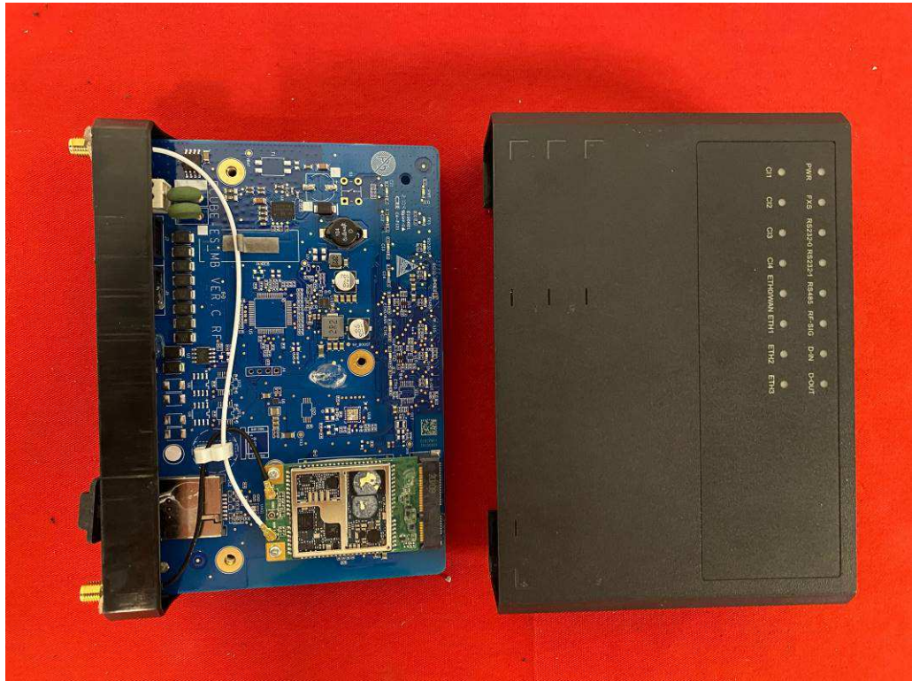
Pic.1 eCube-CP-AU internal view
