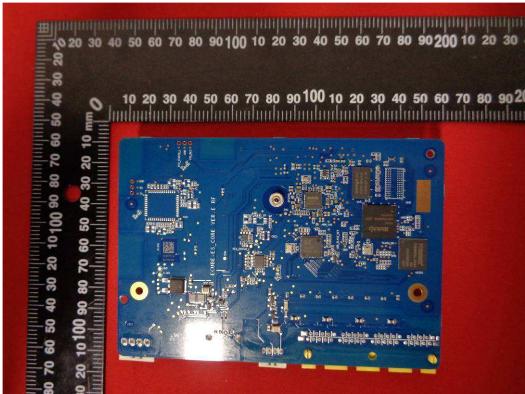
Pic.3 eCube-CP-AU bottom view of PCB 1
