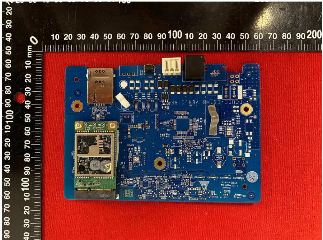
Pic.9 eCube-CG-AU top view of PCB 1
