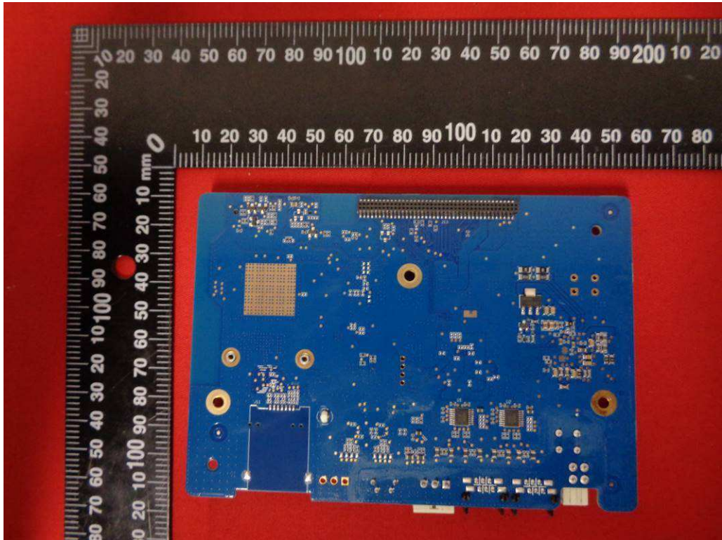
Pic.5 eCube-CP-AU bottom view of PCB 2
