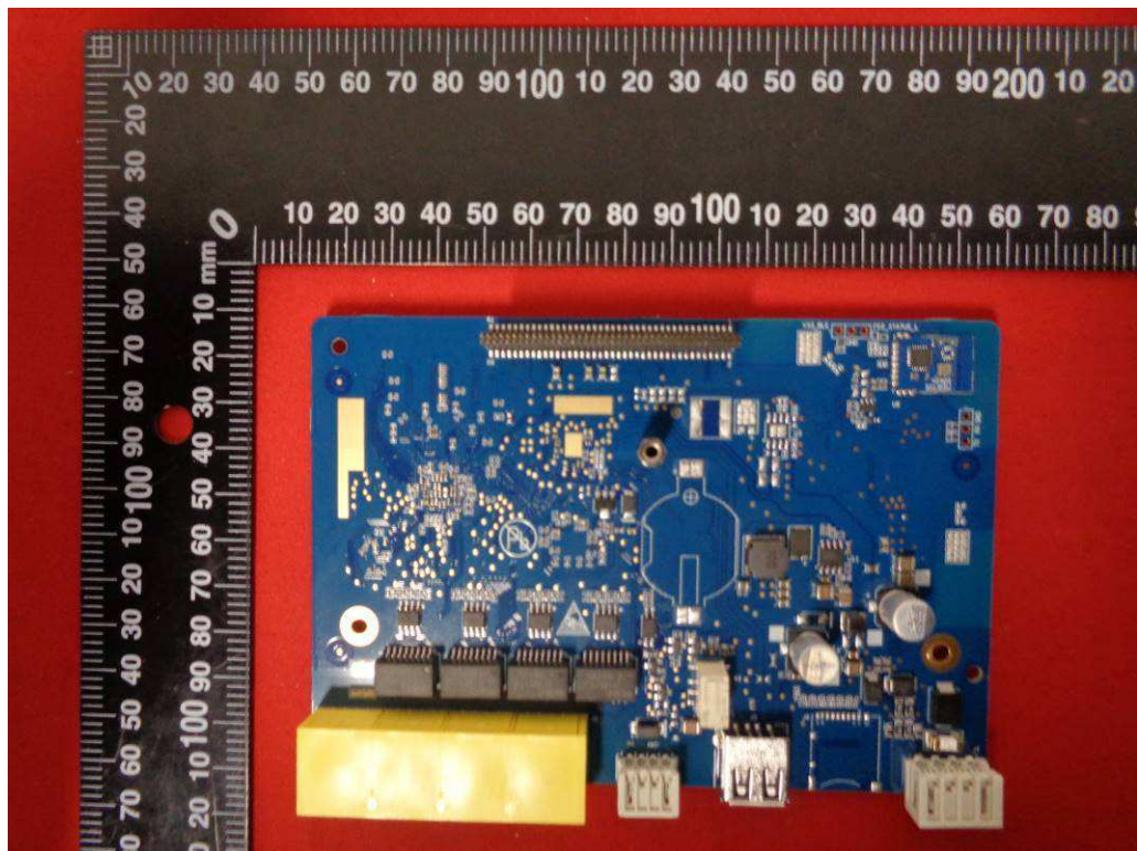
Pic.2 eCube-CP-AU top view of PCB 1
