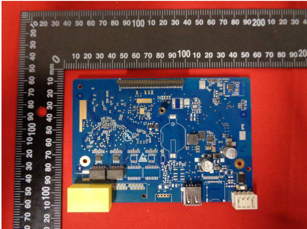
Pic.11 eCube-CG-AU top view of PCB 2
