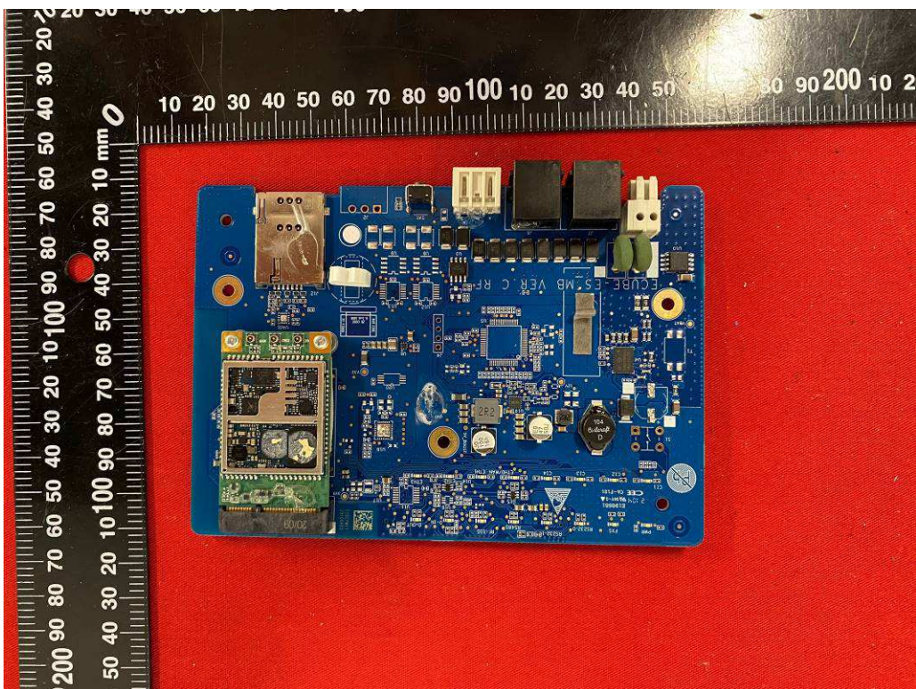
Pic.4 eCube-CP-AU top view of PCB 2
