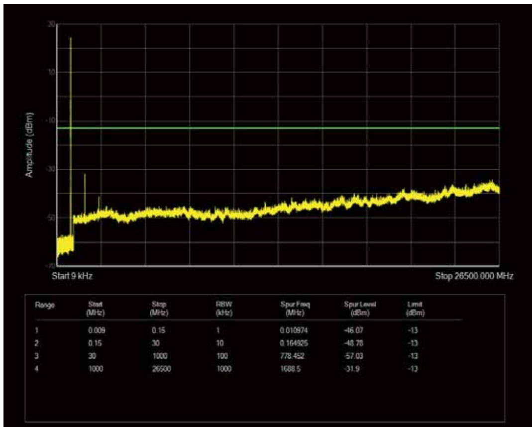
Band26b QPSK BW=3MHz Channel=27025 RB Size=15 Position=#0
