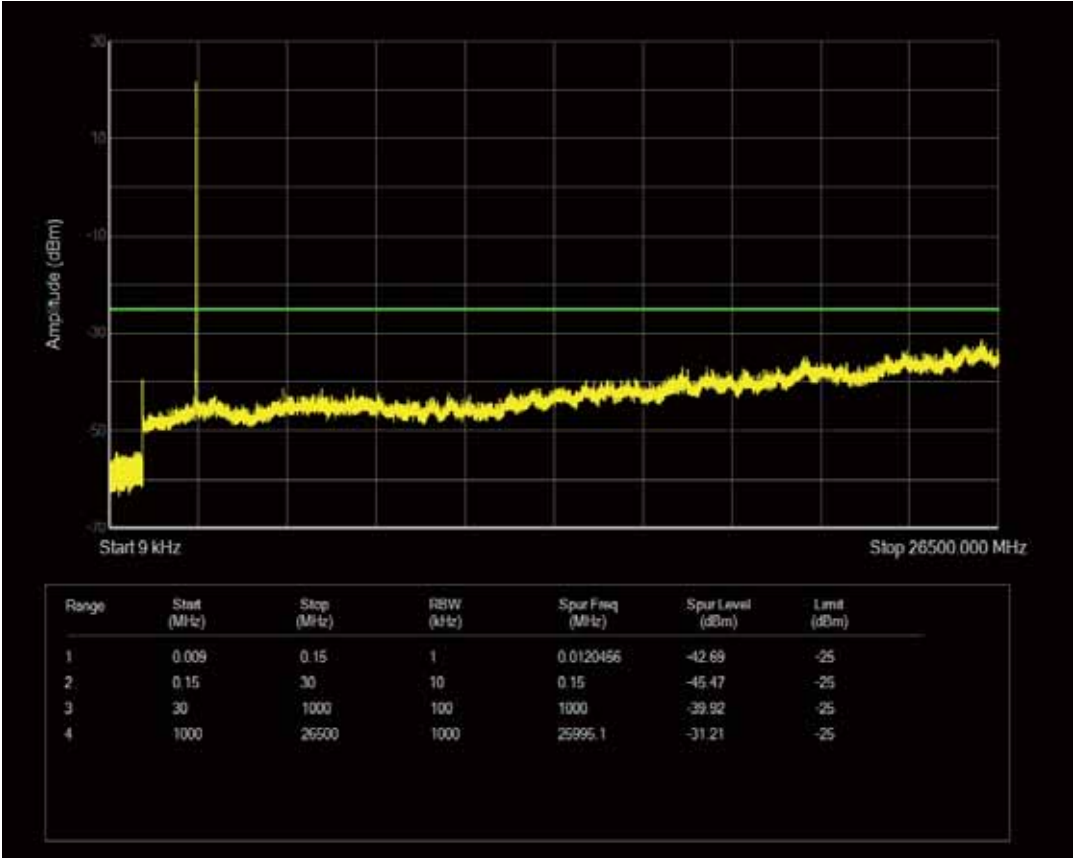
Band41 QAM16 BW=5MHz Channel=40065 RB Size=25 Position=#0
