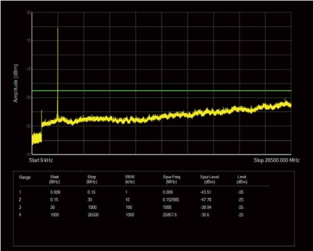
Band41 QAM16 BW=10MHz Channel=40090 RB Size=1 Position=#0
