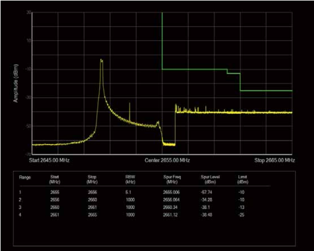
Band41 QPSK BW=5MHz Channel=41215 RB Size=1 Position=#Max
