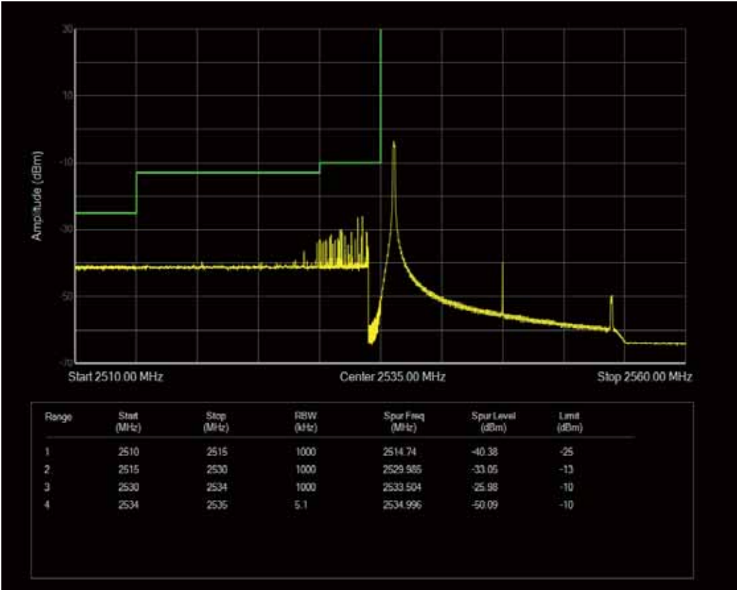
Band41 QAM16 BW=20MHz Channel=40140 RB Size=1 Position=#Max
