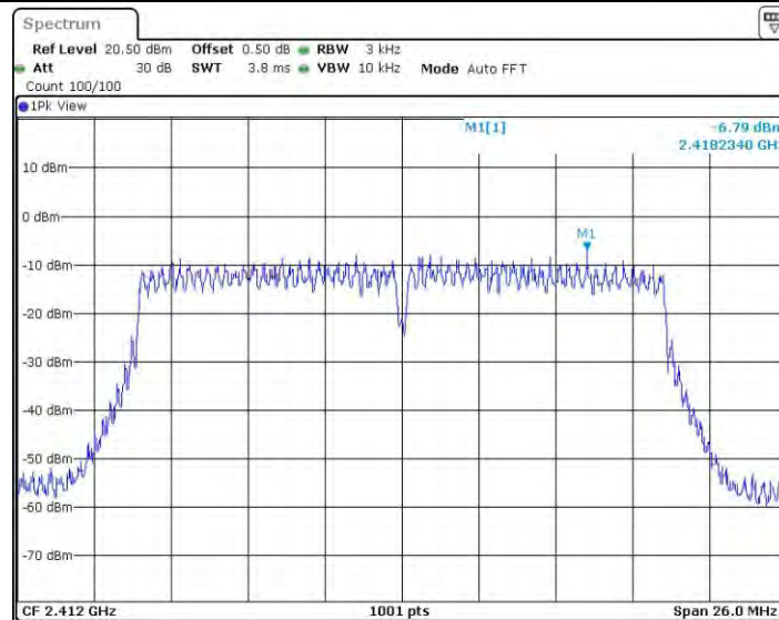
11AC20SISO_Ant0_2412
