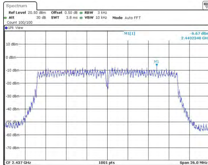
11AC20SISO_Ant1_2437
