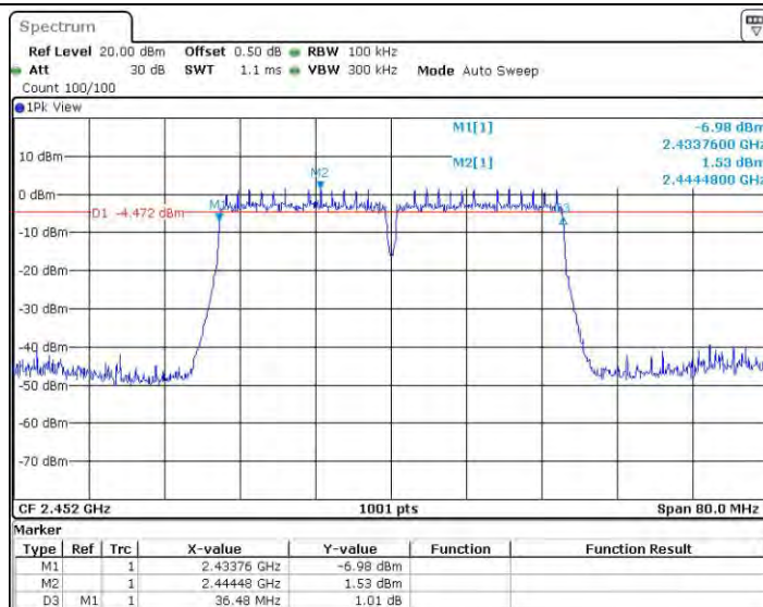
11AC40SISO_Ant1_2452
