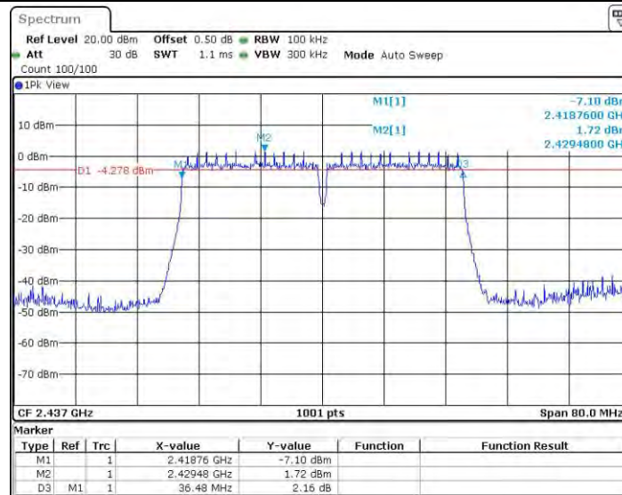
11AC40SISO_Ant1_2437
