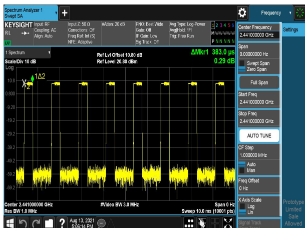
Modulation: \pi/4 DQPSK 2DH1 2441MHz
