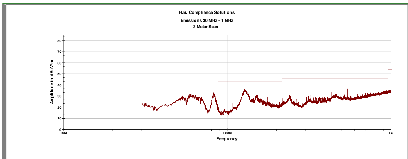
Plot 1 – Radiated Emissions – 30MHz to 1GHz
