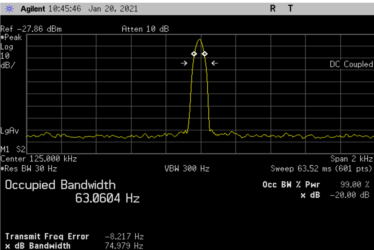
Plot 4 – 20dB BW
