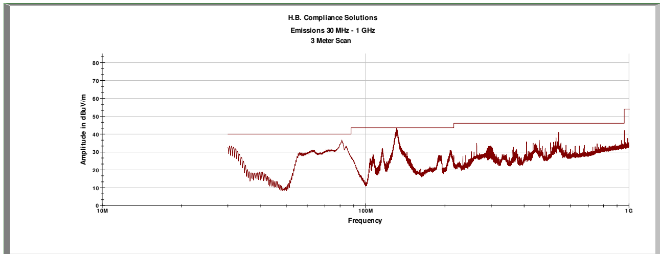
Plot 1 – Radiated Emissions – 30MHz to 1GHz
