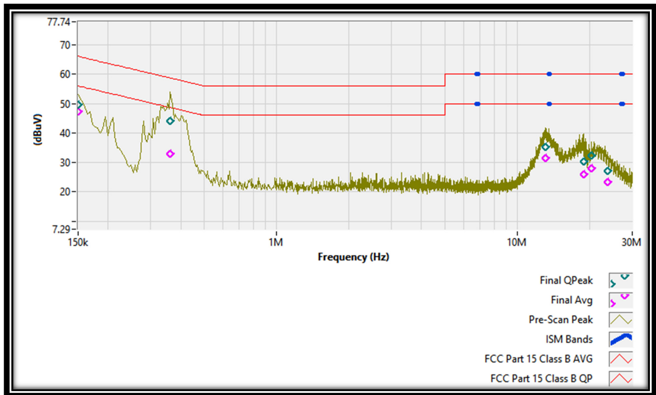
Plot 2 – Conducted Emission Plot – Line Side
