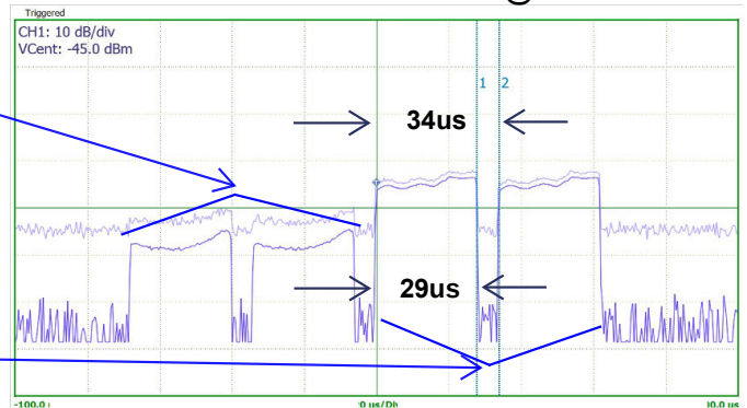
Figure 4.2.1 Example Pulsed Emission Characteristics (Duty Cycle).
