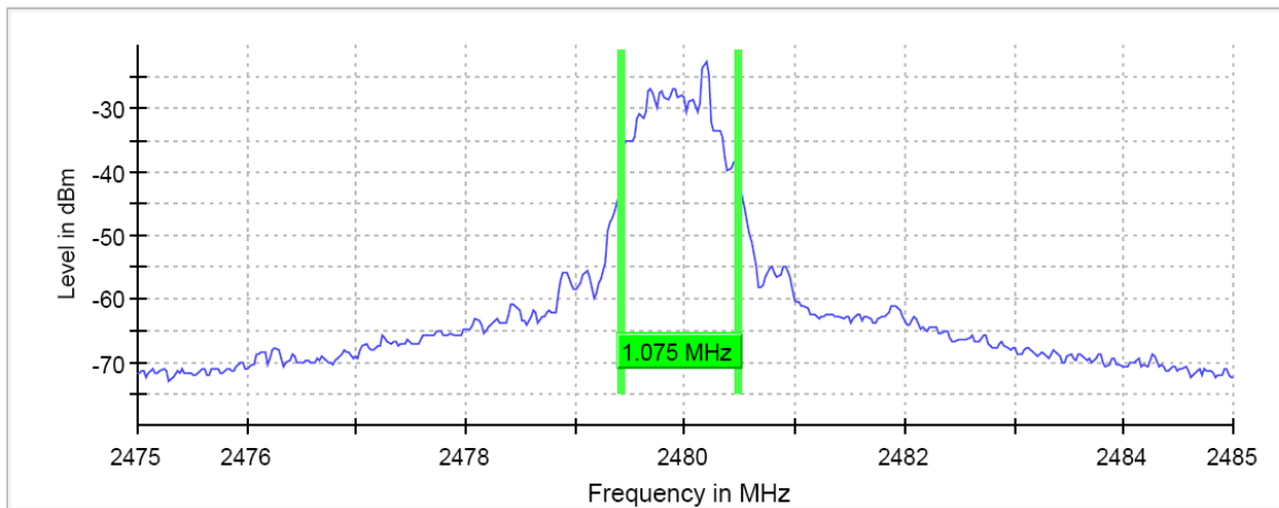
99 % Bandwidth
