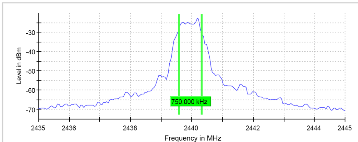
6 dB Bandwidth
