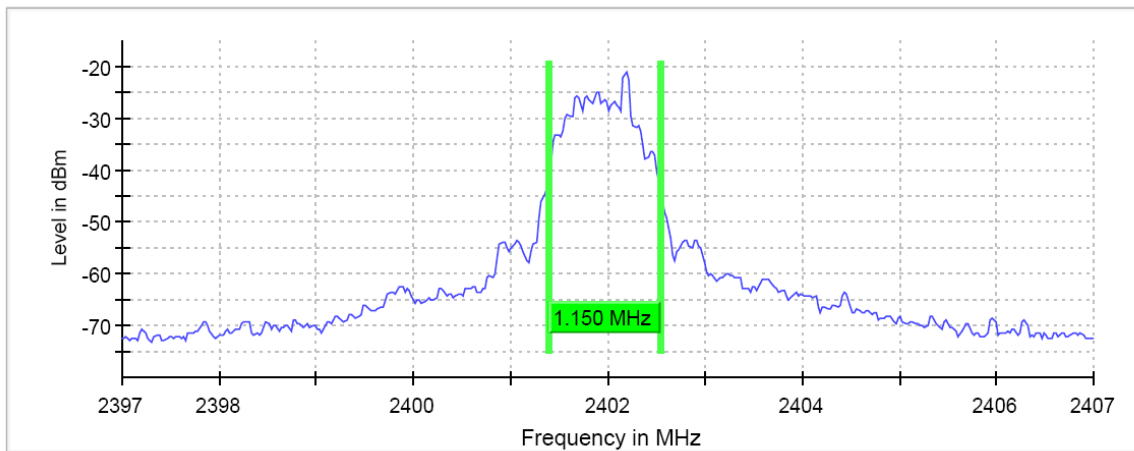
20 dB Bandwidth
