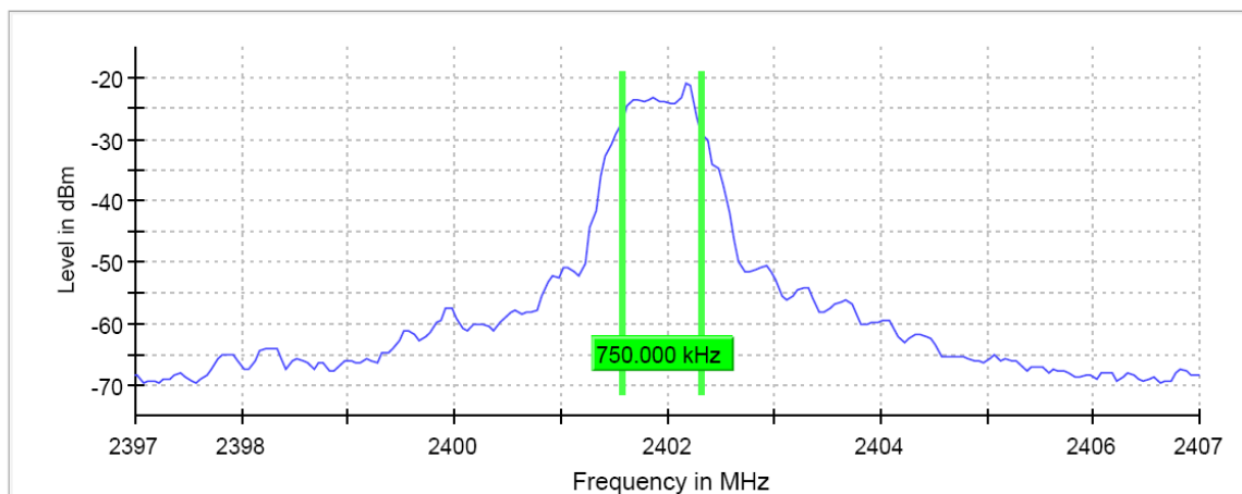
6 dB Bandwidth
