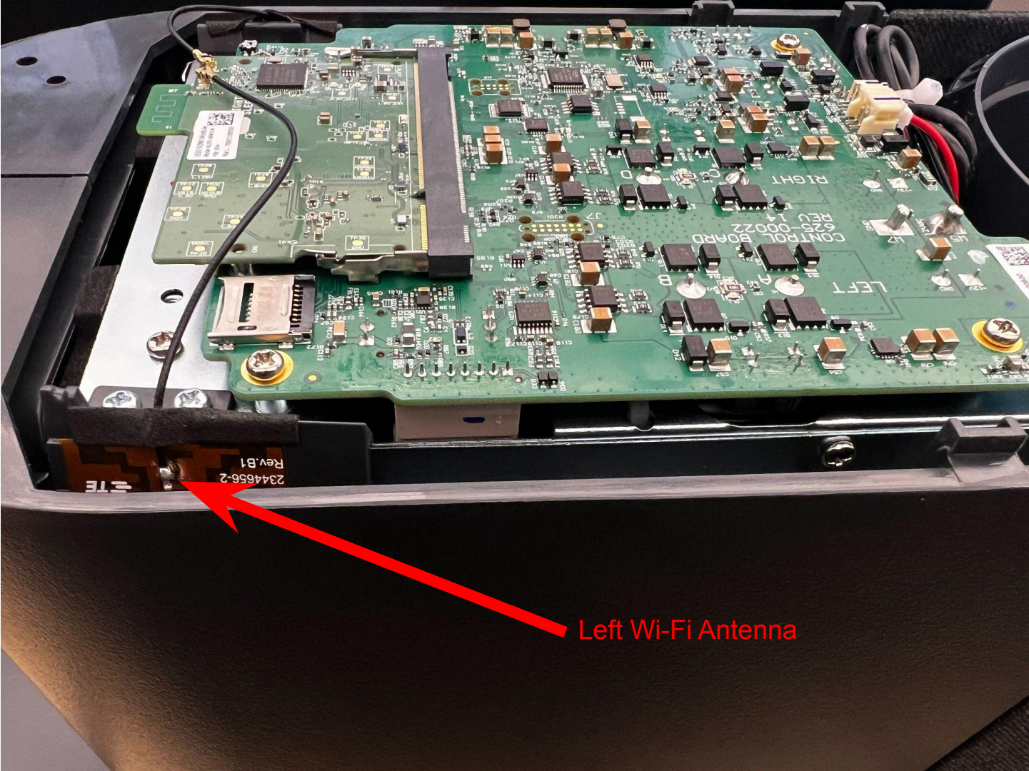
Left Wi-Fi Antenna
