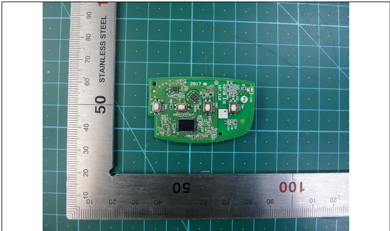
PCB Front
