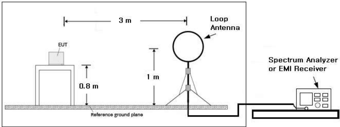
Anechoic Chamber
