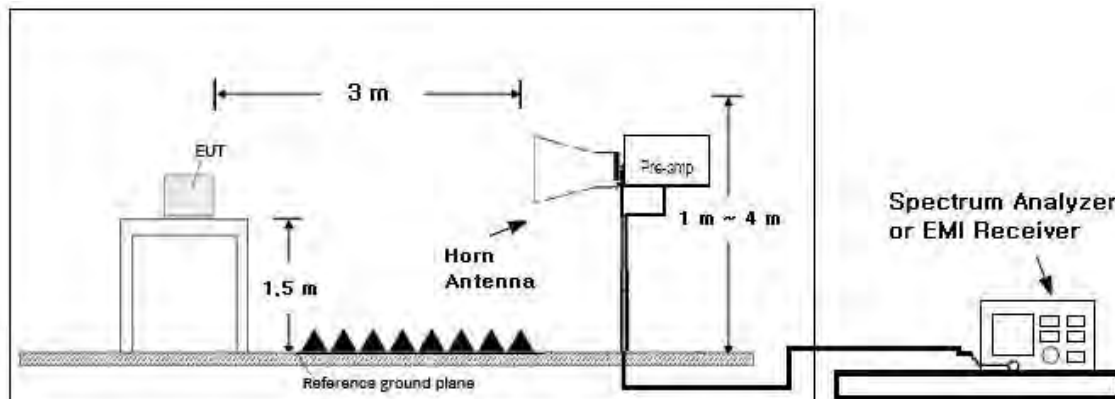
Anechoic Chamber
