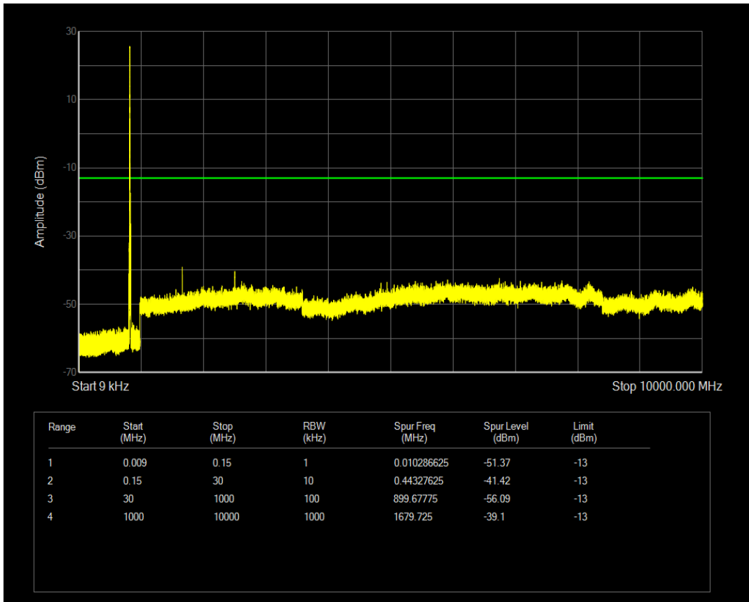
Band5 QAM16 BW=10MHz Channel=20600 RB Size=1 Position=#Mid
