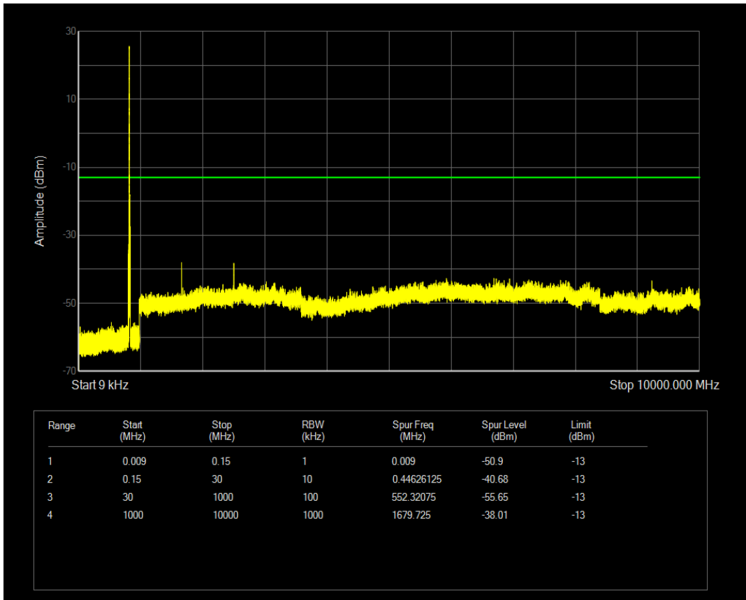
Band5 QPSK BW=10MHz Channel=20600 RB Size=1 Position=#Mid
