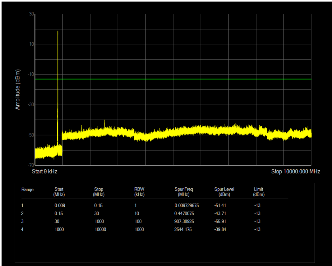
Band5 QAM16 BW=3MHz Channel=20635 RB Size=8 Position=#Max
