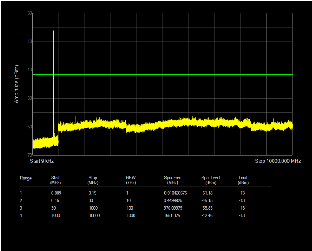
Band5 QPSK BW=3MHz Channel=20415 RB Size=8 Position=#Max
