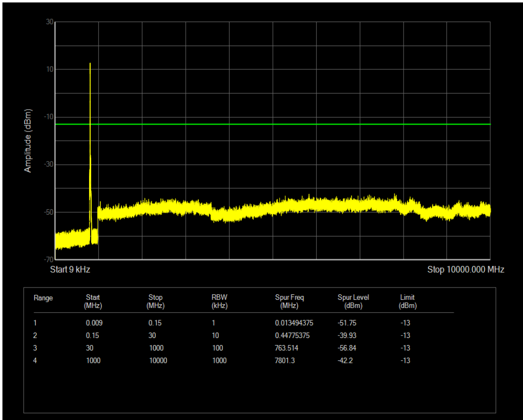
Band5 QAM16 BW=10MHz Channel=20450 RB Size=1 Position=#Mid
