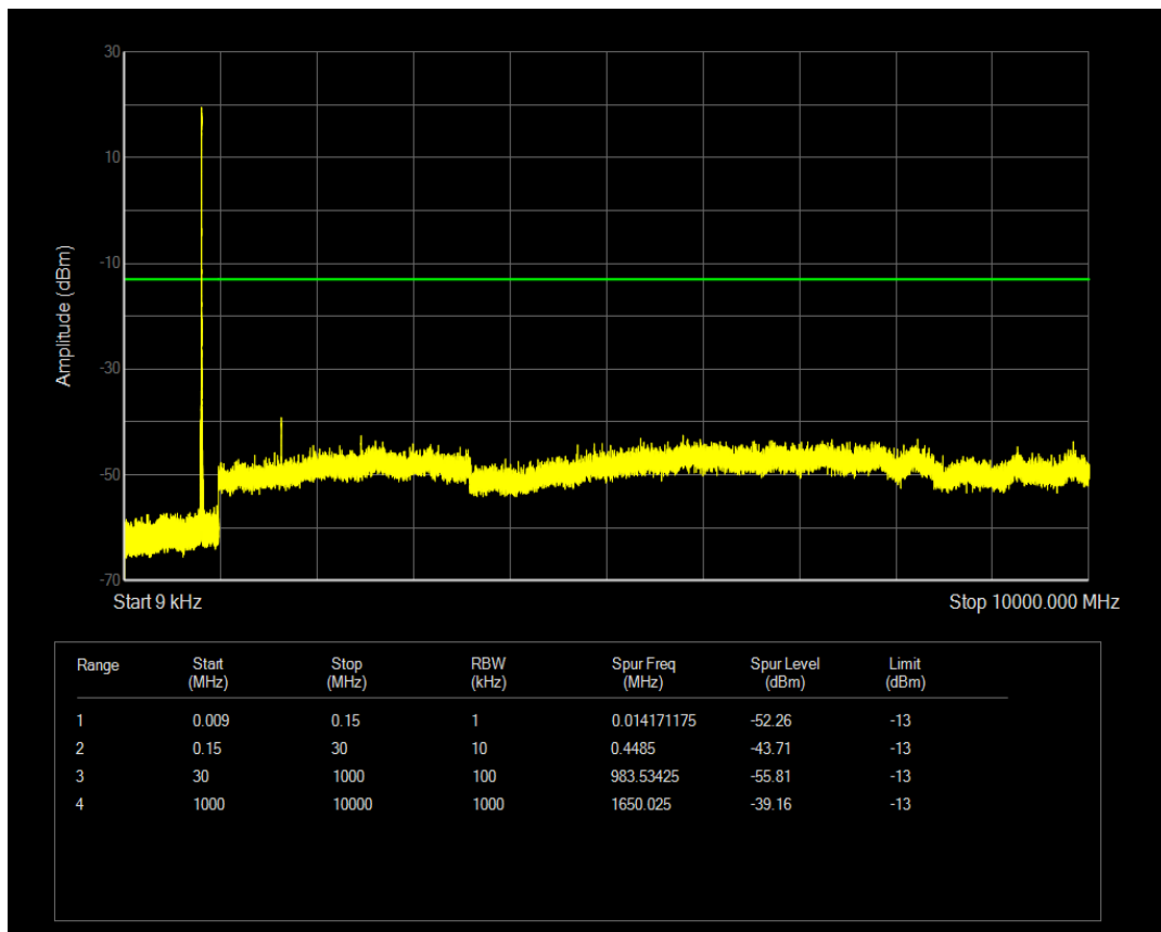
Band5 QAM16 BW=3MHz Channel=20415 RB Size=8 Position=#0
