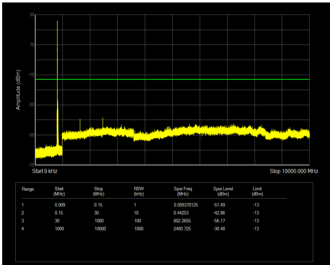
Band5 QAM16 BW=5MHz Channel=20425 RB Size=1 Position=#Mid
