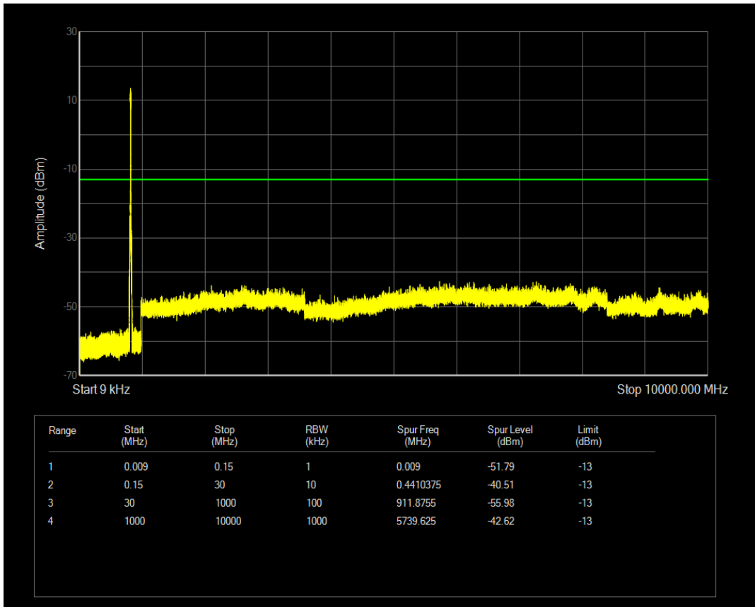
Band5 QAM16 BW=10MHz Channel=20525 RB Size=1 Position=#Mid
