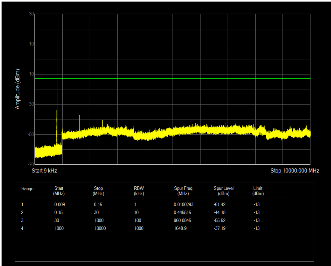
Band5 QAM16 BW=3MHz Channel=20415 RB Size=1 Position=#Mid
