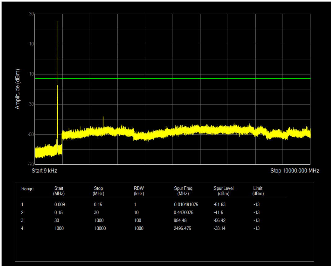
Band5 QPSK BW=10MHz Channel=20525 RB Size=1 Position=#Mid
