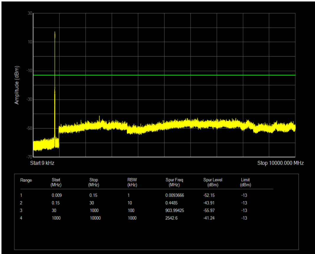
Band5 QAM16 BW=3MHz Channel=20635 RB Size=8 Position=#Max
