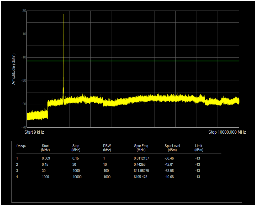
Band4 QAM16 BW=15MHz Channel=20175 RB Size=1 Position=#Mid
