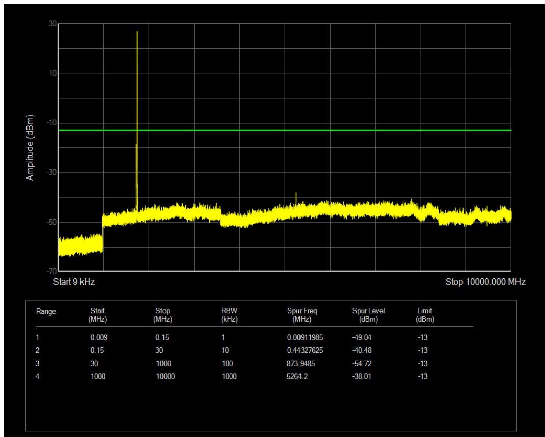
Band4 QAM16 BW=5MHz Channel=20375 RB Size=12 Position=#0
