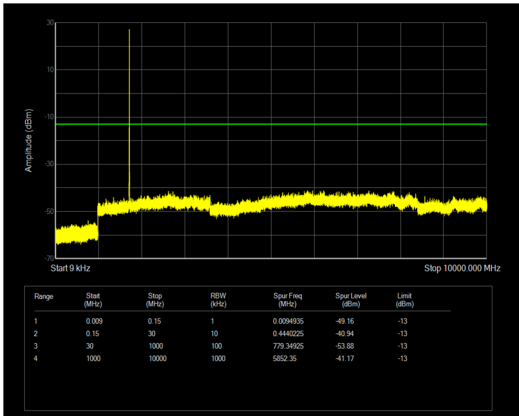
Band4 QAM16 BW=3MHz Channel=20175 RB Size=8 Position=#0
