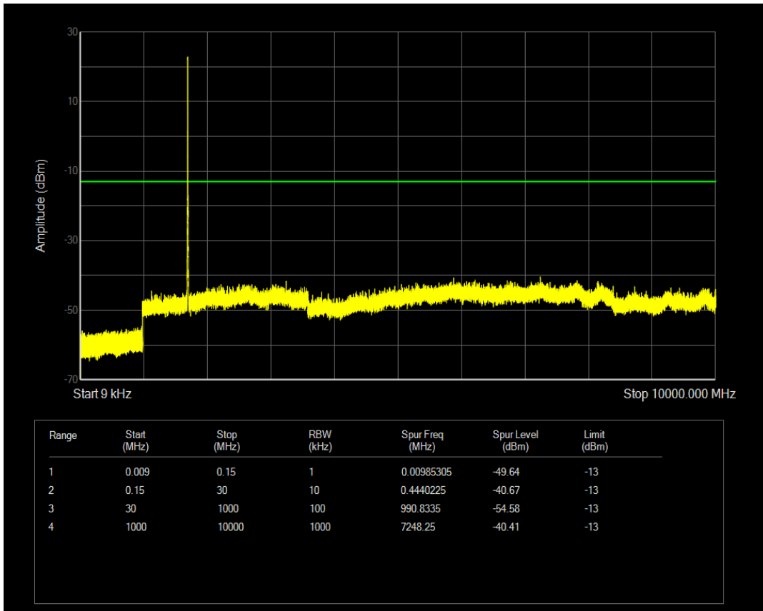
Band4 QPSK BW=5MHz Channel=19975 RB Size=12 Position=#0
