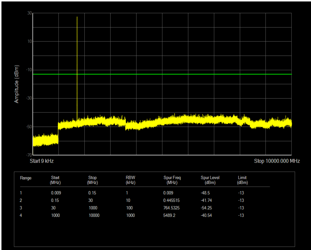
Band4 QPSK BW=1.4MHz Channel=20175 RB Size=3 Position=#0
