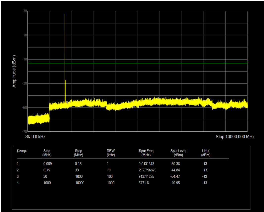
Band4 QAM16 BW=1.4MHz Channel=19957 RB Size=1 Position=#Mid
