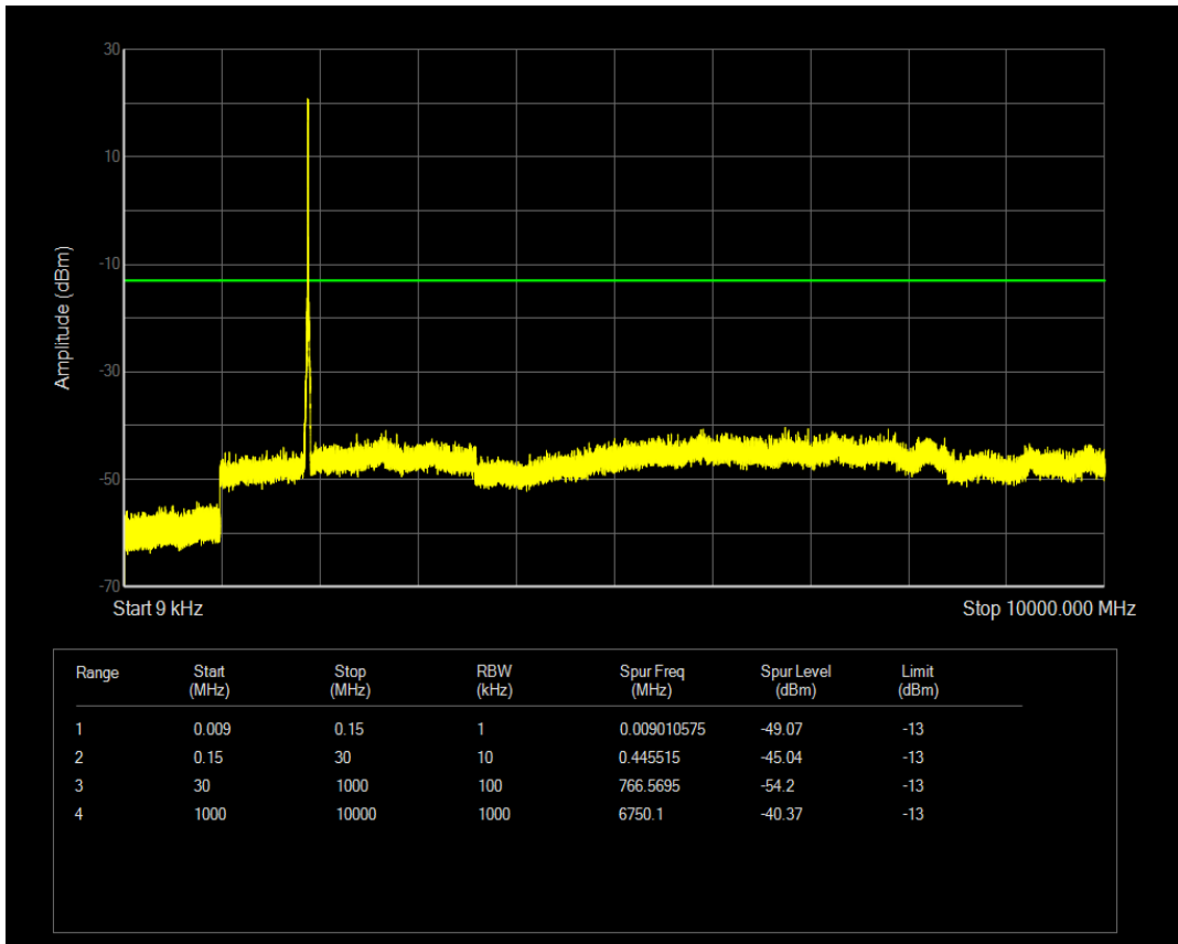
Band2 QAM16 BW=20MHz Channel=19100 RB Size=50 Position=#0
