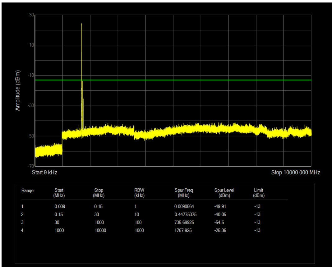
Band4 QPSK BW=3MHz Channel=19965 RB Size=8 Position=#0
