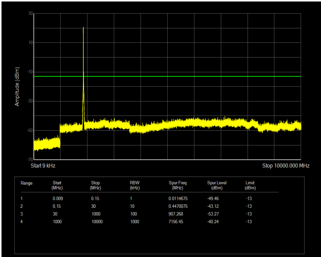
Band2 QAM16 BW=20MHz Channel=18900 RB Size=50 Position=#0
