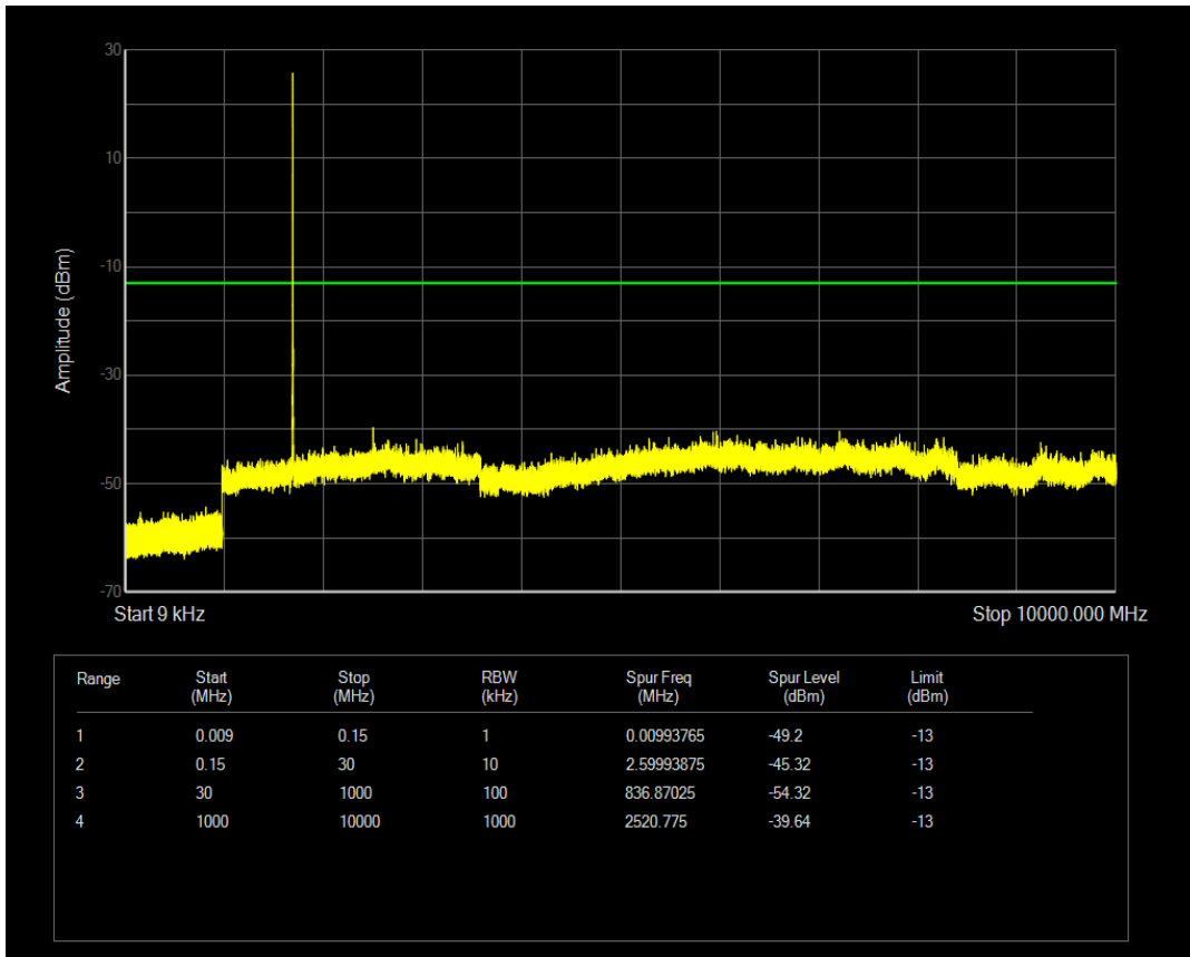
Band4 QAM16 BW=1.4MHz Channel=19957 RB Size=1 Position=#Mid
