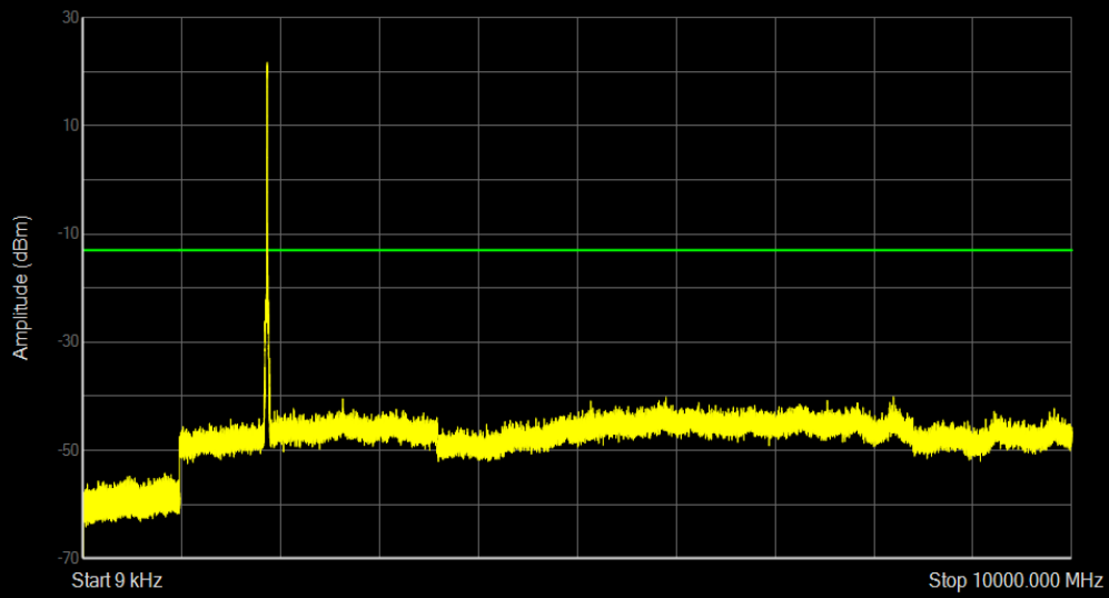
Band2 QPSK BW=15MHz Channel=18900 RB Size=36 Position=#Max
