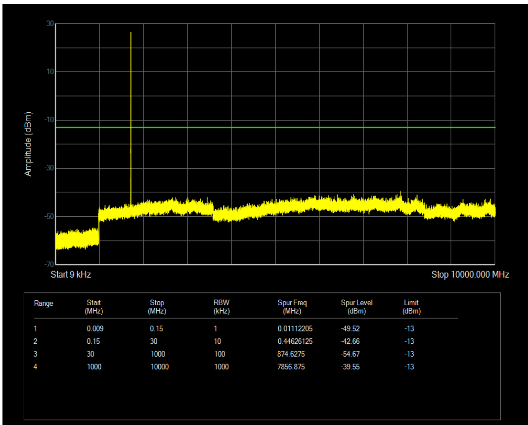
Band4 QAM16 BW=1.4MHz Channel=20175 RB Size=3 Position=#Max
