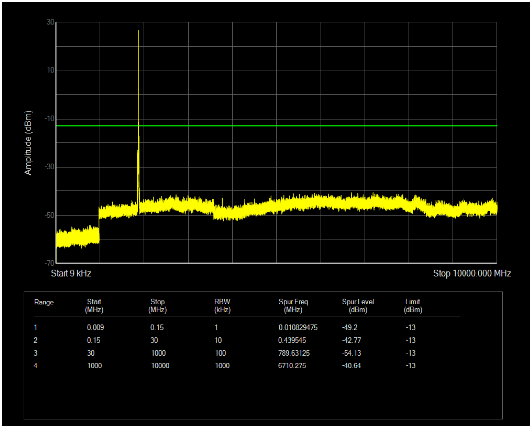
Band2 QPSK BW=15MHz Channel=19125 RB Size=1 Position=#Mid
