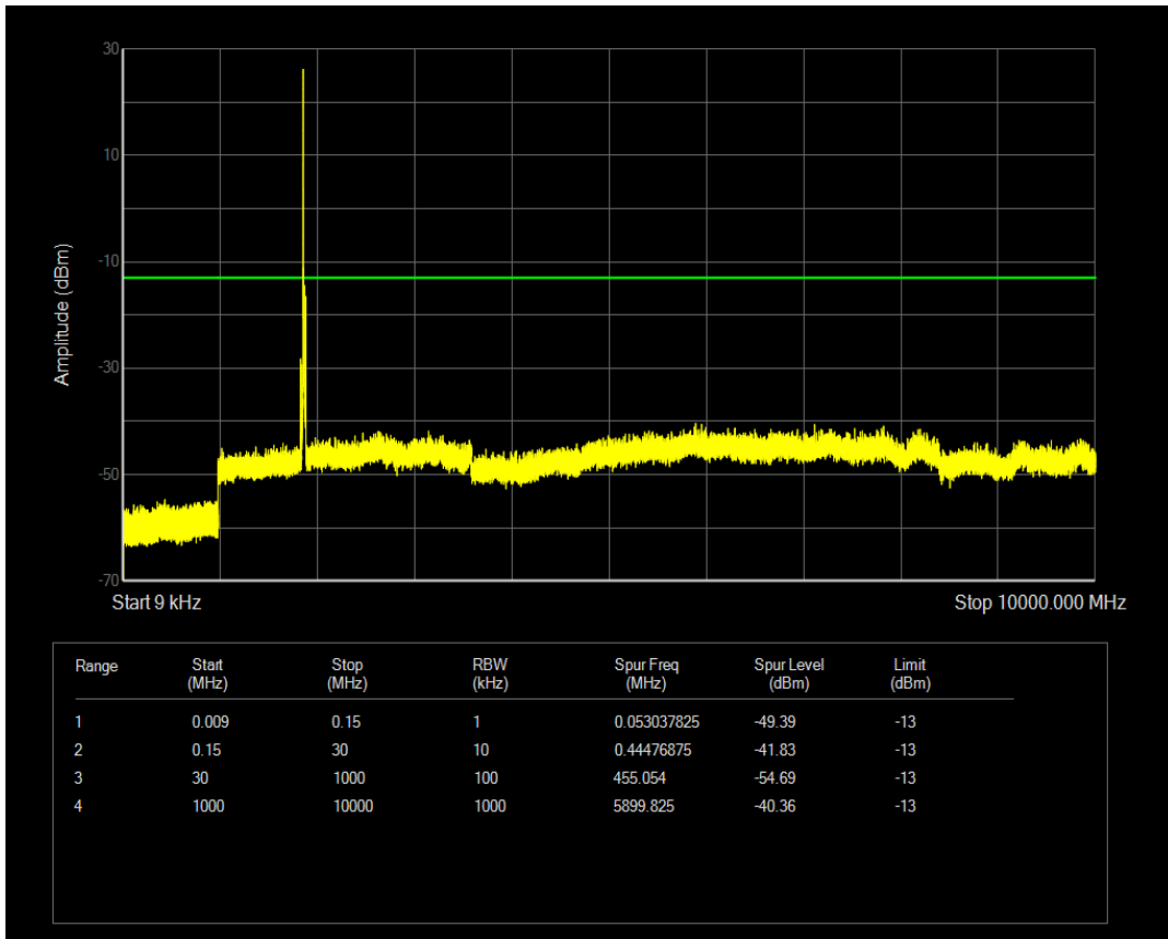
Band2 QAM16 BW=15MHz Channel=18900 RB Size=1 Position=#Mid
