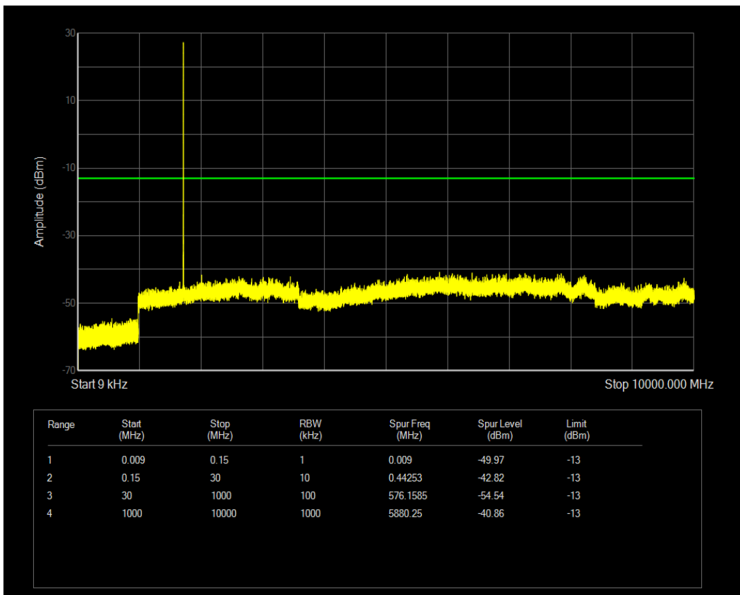
Band4 QPSK BW=1.4MHz Channel=20175 RB Size=3 Position=#0
