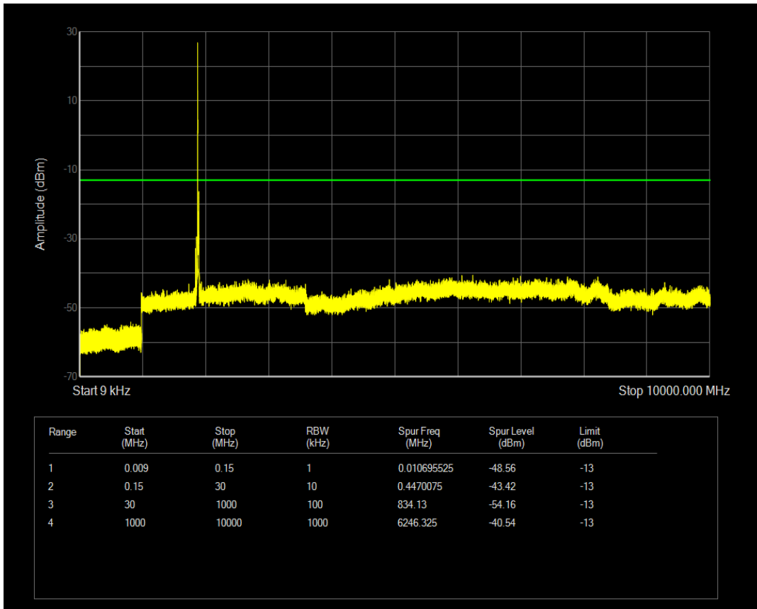
Band2 QAM16 BW=20MHz Channel=19100 RB Size=1 Position=#Mid
