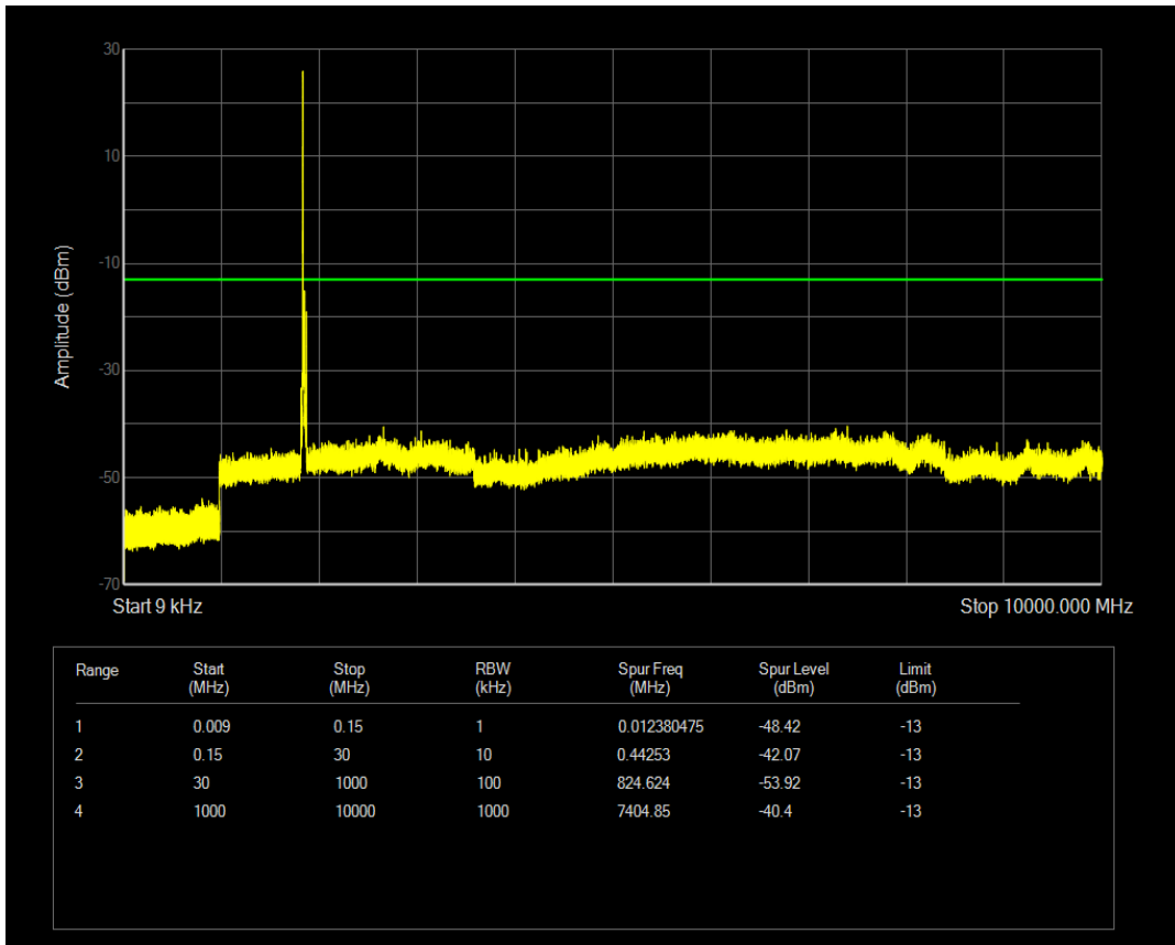
Band2 QAM16 BW=20MHz Channel=18700 RB Size=1 Position=#Mid
