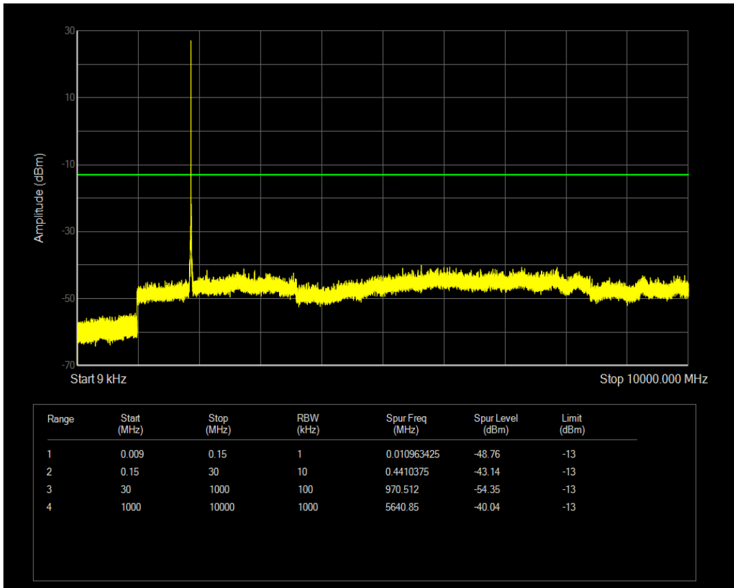
Band2 QAM16 BW=20MHz Channel=18900 RB Size=1 Position=#Mid
