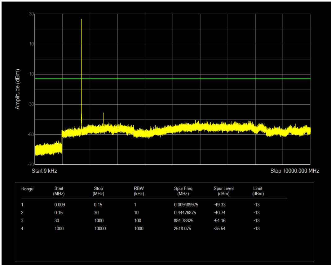
Band4 QAM16 BW=3MHz Channel=19965 RB Size=1 Position=#Mid
