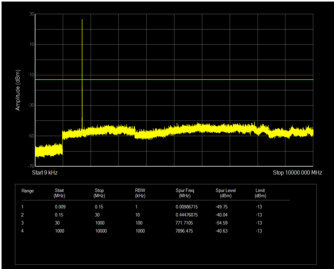
Band4 QAM16 BW=3MHz Channel=19965 RB Size=1 Position=#Mid
