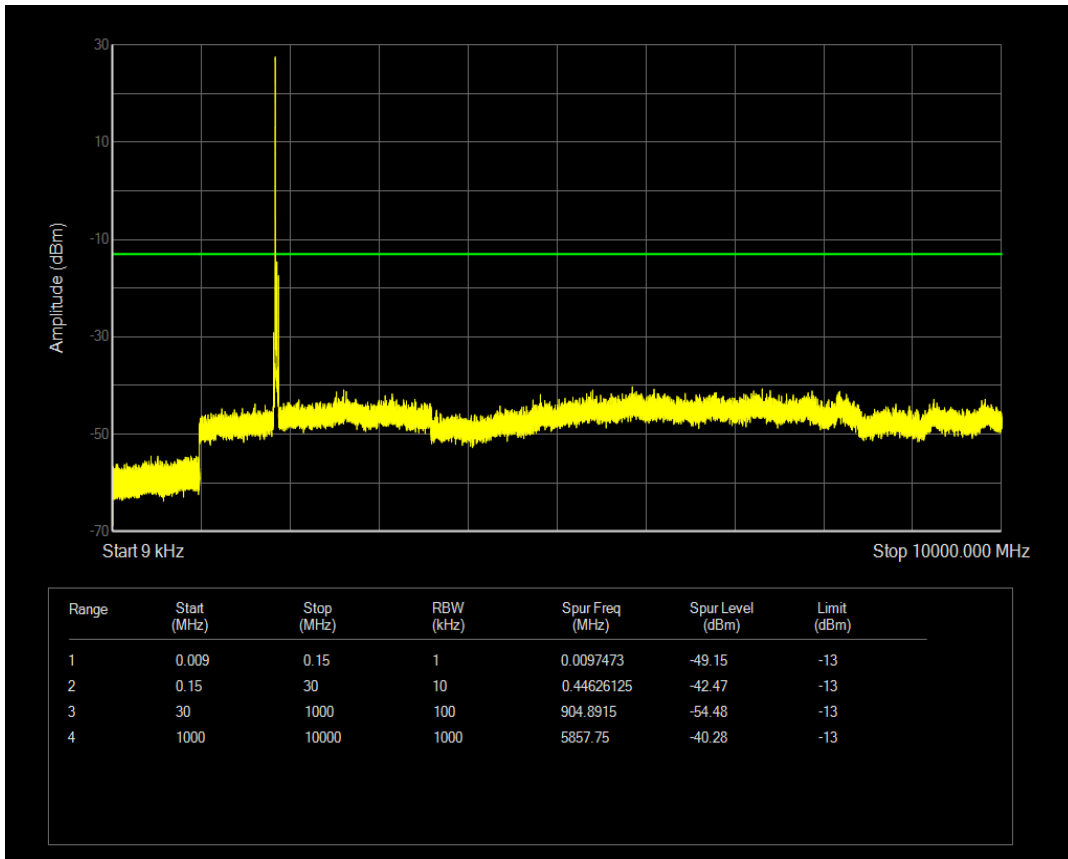
Band2 QPSK BW=20MHz Channel=18700 RB Size=1 Position=#Mid
