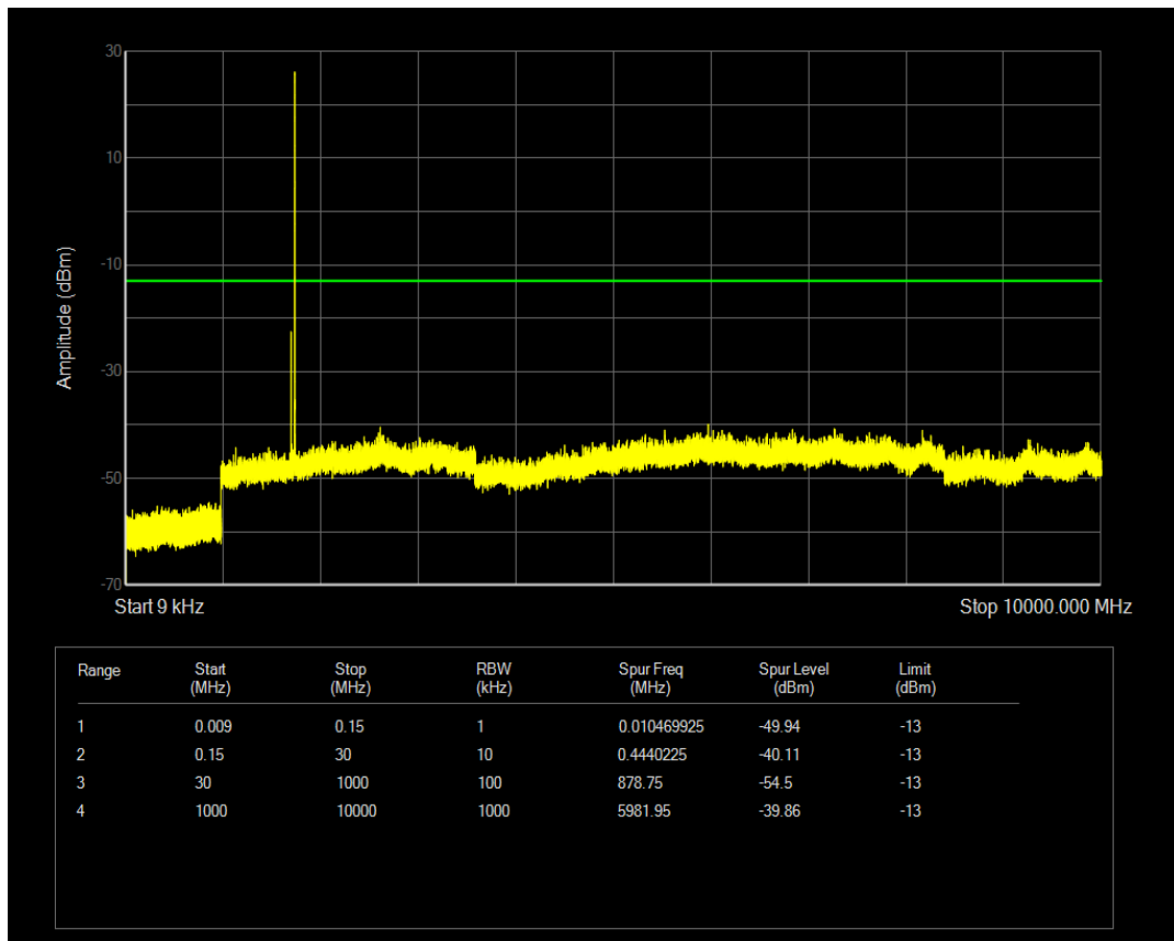
Band4 QPSK BW=1.4MHz Channel=20393 RB Size=3 Position=#0
