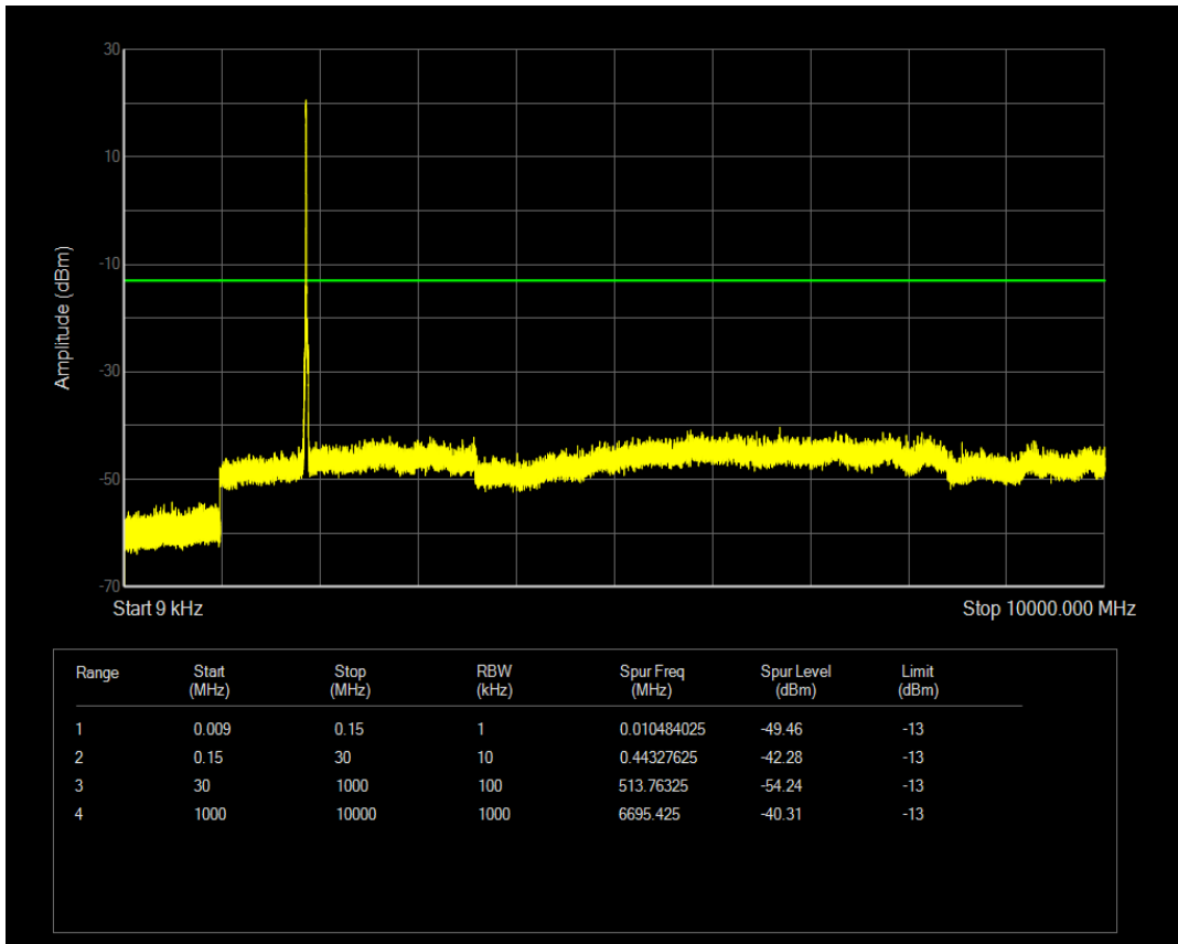
Band2 QAM16 BW=15MHz Channel=18900 RB Size=36 Position=#0
