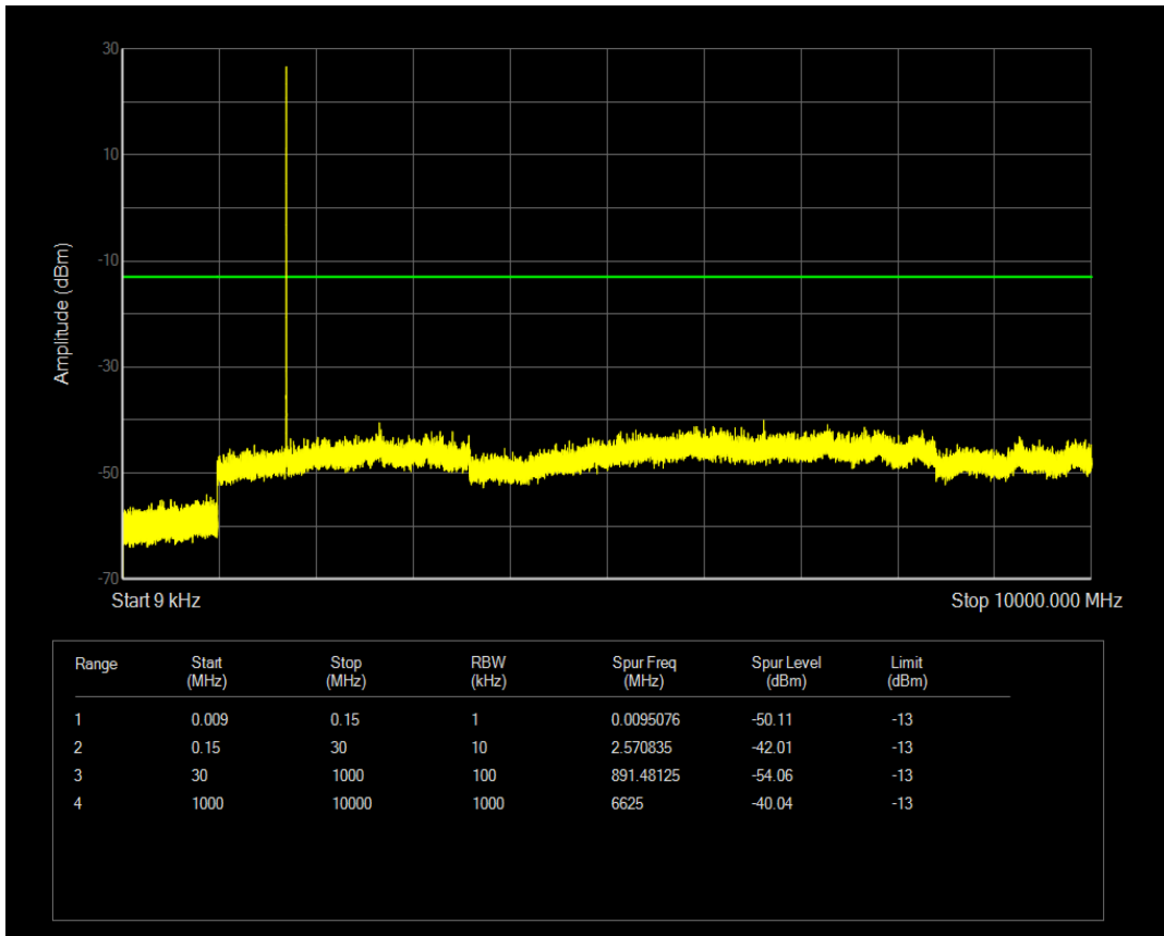
Band4 QPSK BW=1.4MHz Channel=19957 RB Size=1 Position=#Mid
