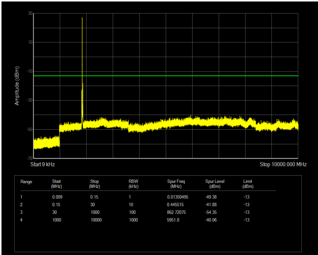
Band2 QAM16 BW=20MHz Channel=18700 RB Size=1 Position=#Mid
