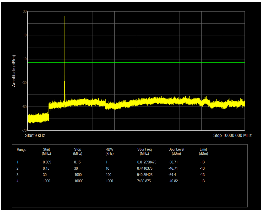
Band4 QPSK BW=1.4MHz Channel=19957 RB Size=3 Position=#0
