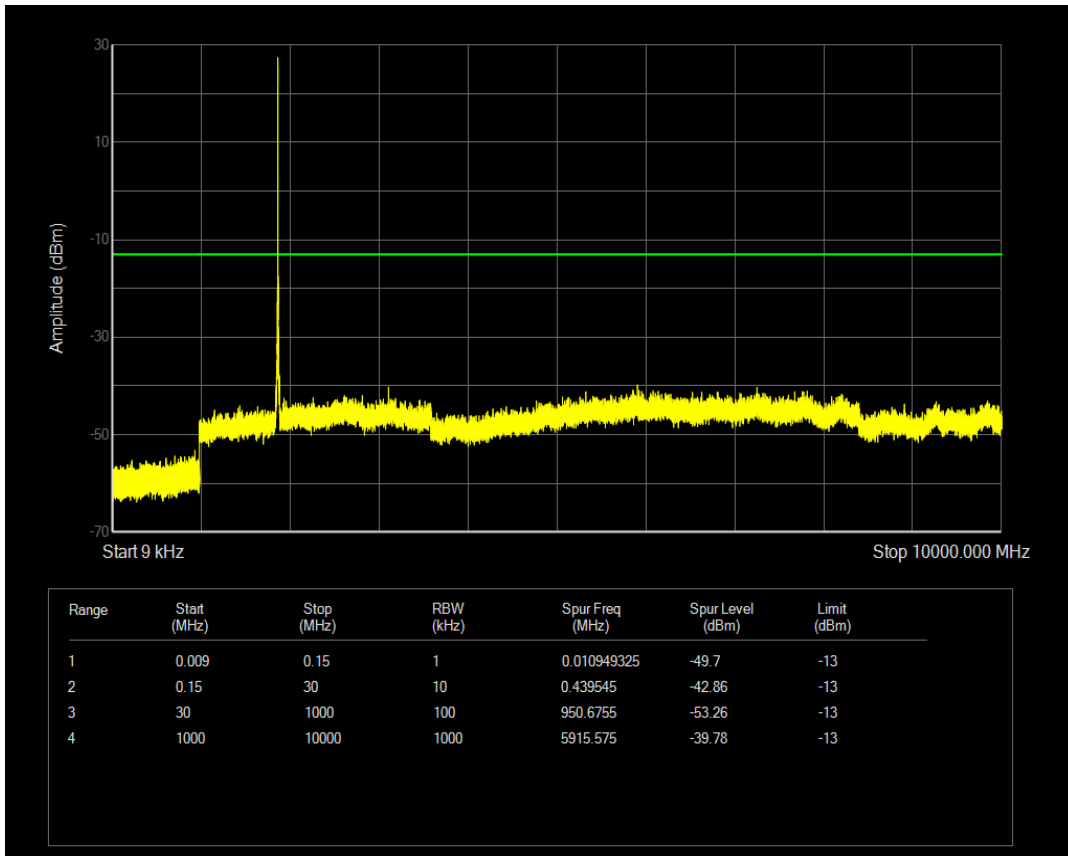
Band2 QAM16 BW=15MHz Channel=18900 RB Size=1 Position=#Mid
