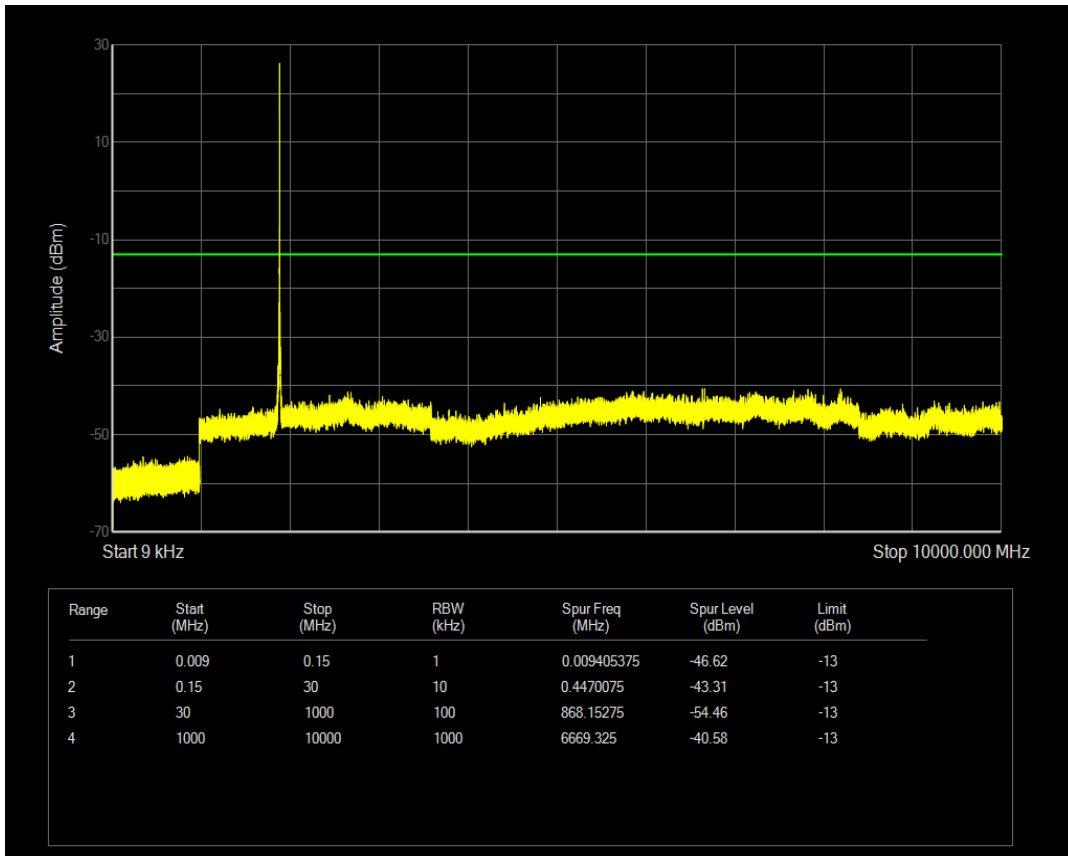
Band2 QPSK BW=20MHz Channel=19100 RB Size=1 Position=#Mid
