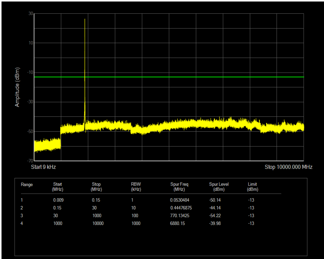
Band2 QAM16 BW=20MHz Channel=19100 RB Size=1 Position=#Mid
