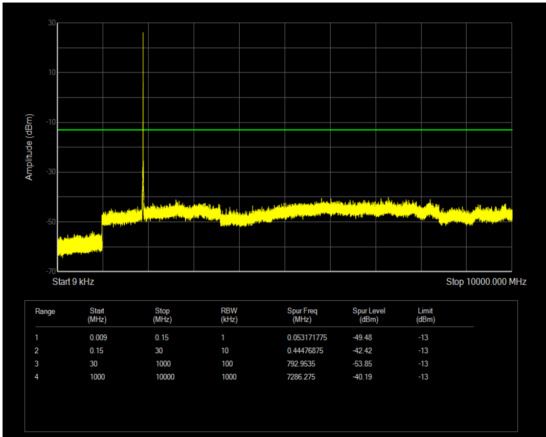
Band2 QAM16 BW=15MHz Channel=19125 RB Size=1 Position=#Mid
