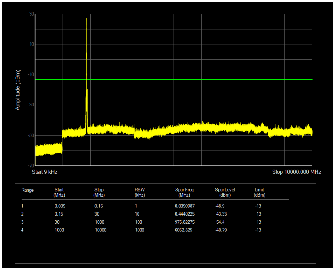
Band2 QAM16 BW=20MHz Channel=18900 RB Size=1 Position=#Mid
