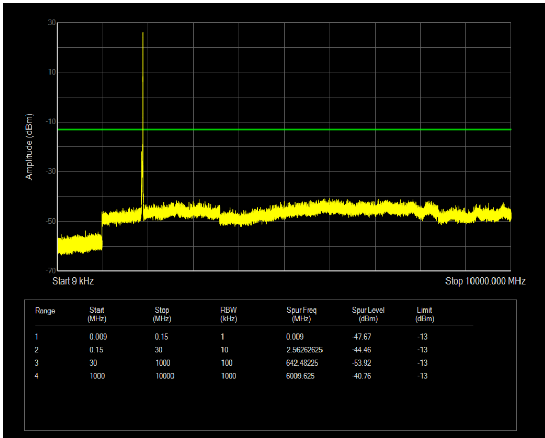
Band2 QAM16 BW=20MHz Channel=19100 RB Size=50 Position=#0
