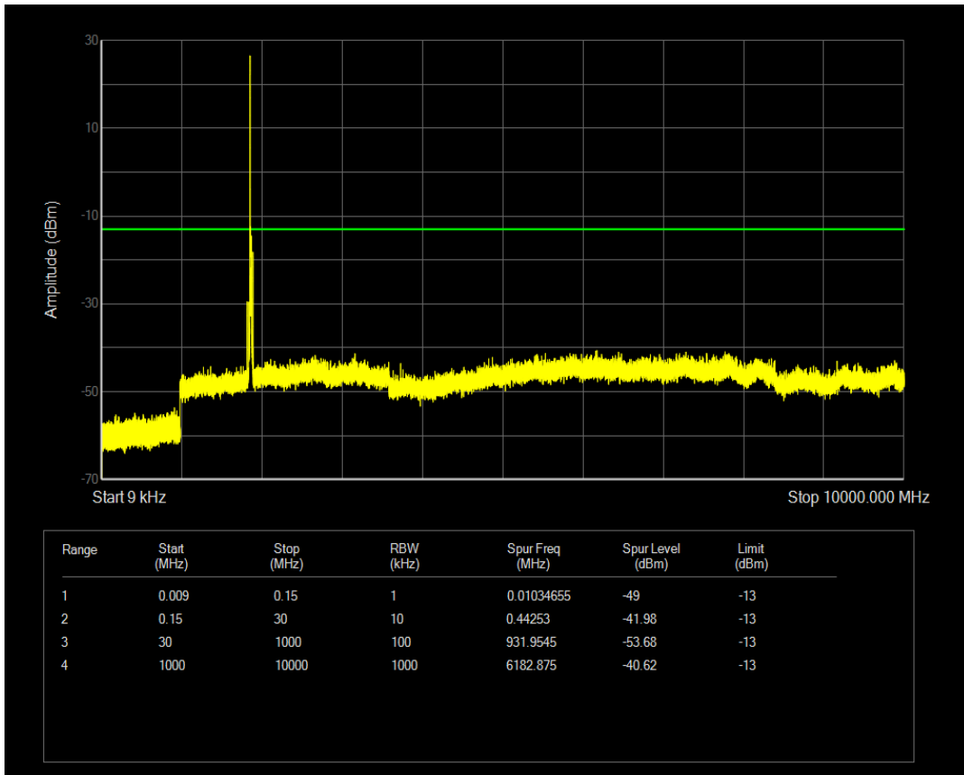
Band2 QPSK BW=20MHz Channel=18900 RB Size=1 Position=#Mid
