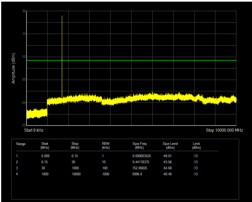
Band4 QAM16 BW=1.4MHz Channel=19957 RB Size=3 Position=#0
