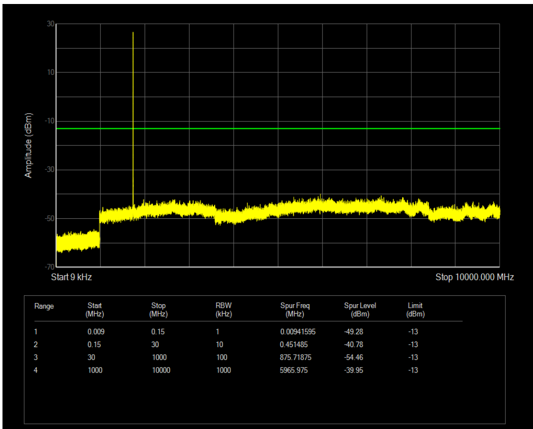
Band4 QAM16 BW=1.4MHz Channel=20393 RB Size=3 Position=#Max
