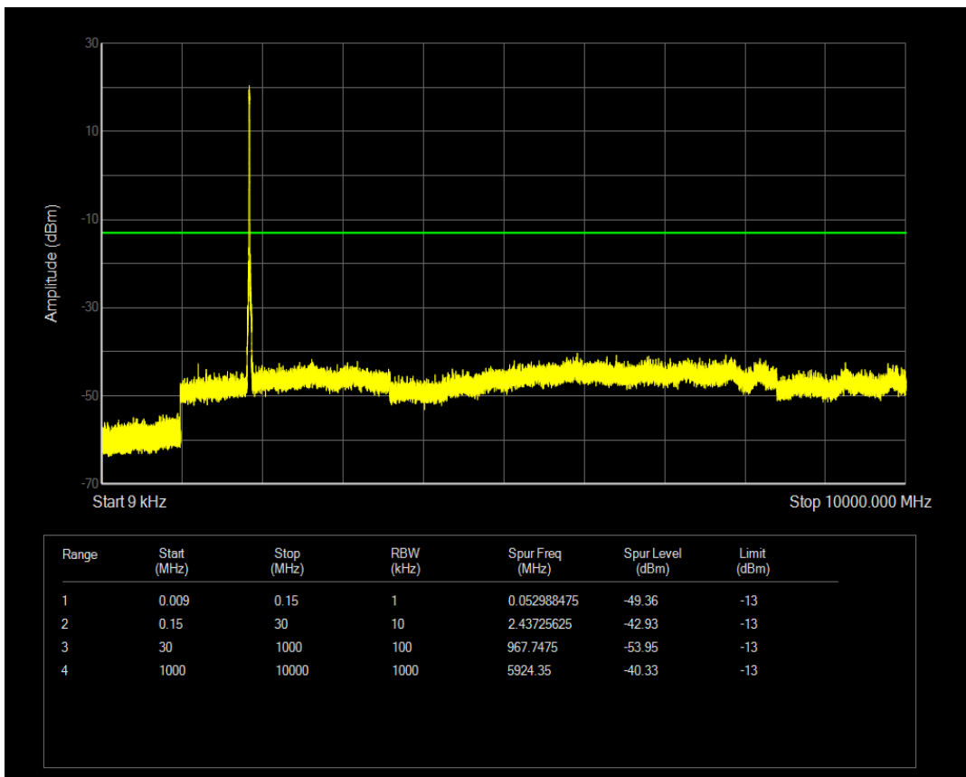
Band2 QAM16 BW=20MHz Channel=18700 RB Size=50 Position=#0
