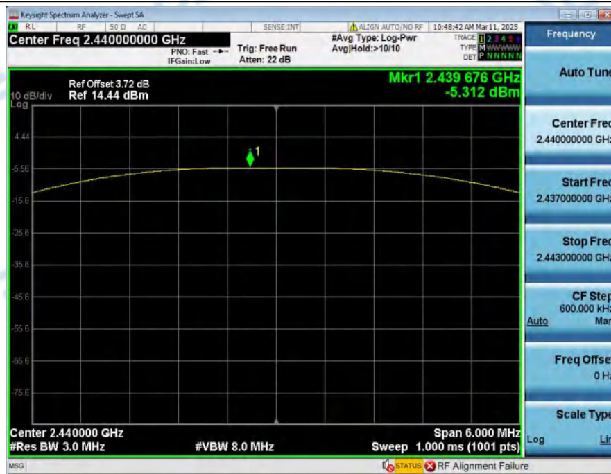
Peak_Output_Power_NVNT_ANT1_2Mbps_2440
