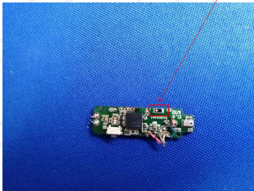
BT Antenna
