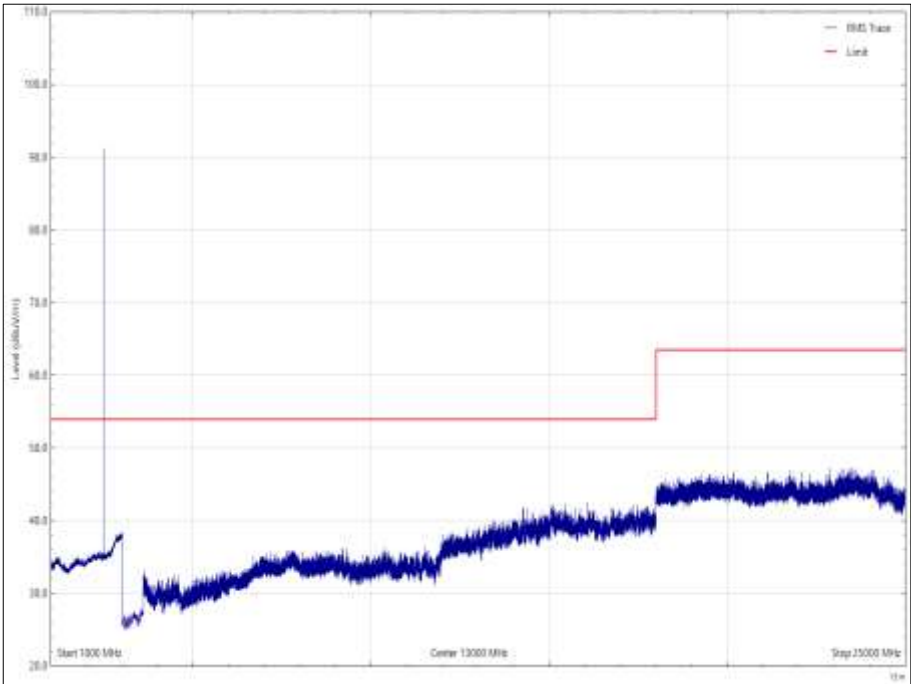
Figure 59 - 2480 MHz, 1 GHz to 25 GHz, Horizontal and Vertical, Z Orientation, Average
