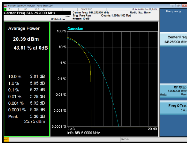
64QAM-20635
