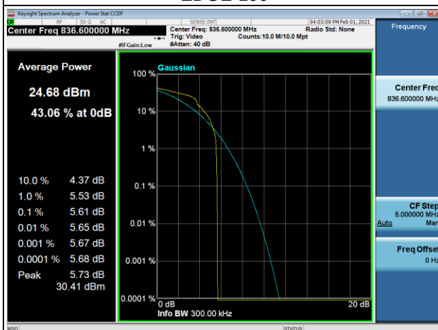
EDGE-190
