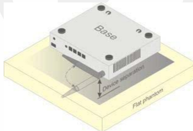
Fig-4.1 Device with swivel antenna
