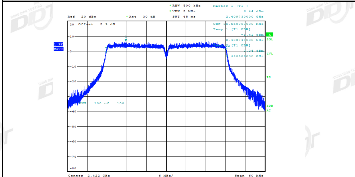
11N40SISO Ant1_2422
