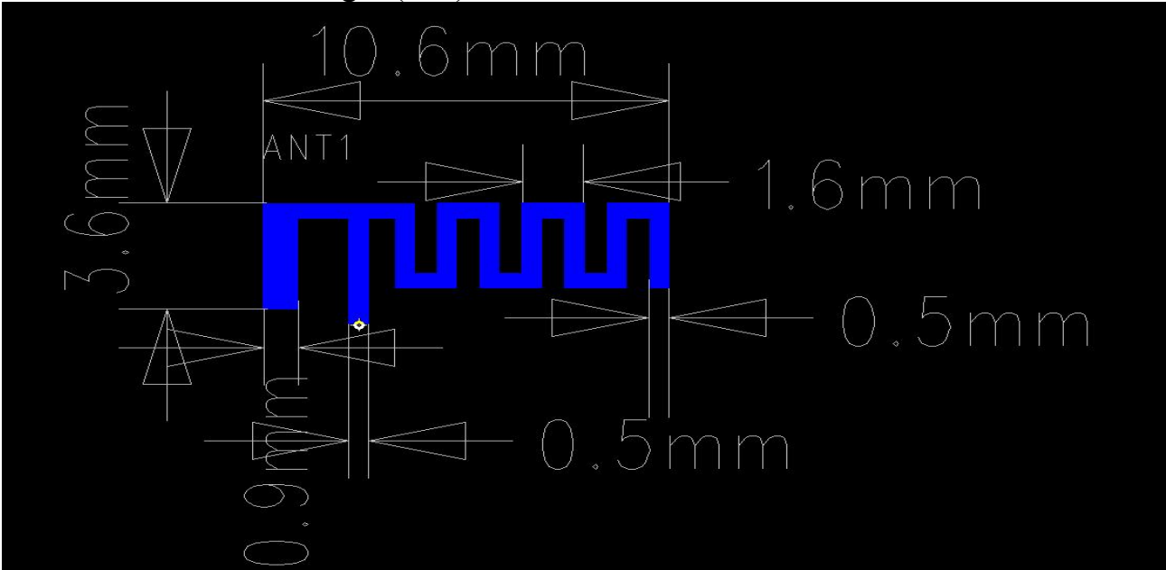
Antenna Photo & Length (mm)
