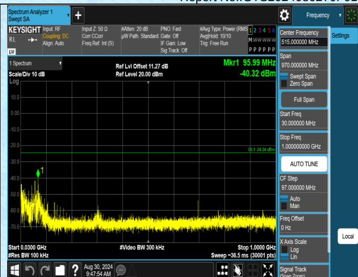
2DH5-Ant1-2441-30~1000-PASS
