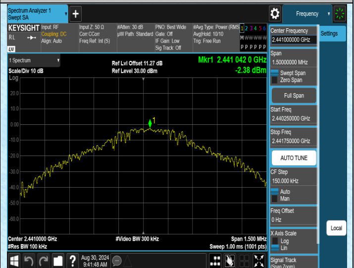
DH5-Ant1-2441-0~Reference-PASS
