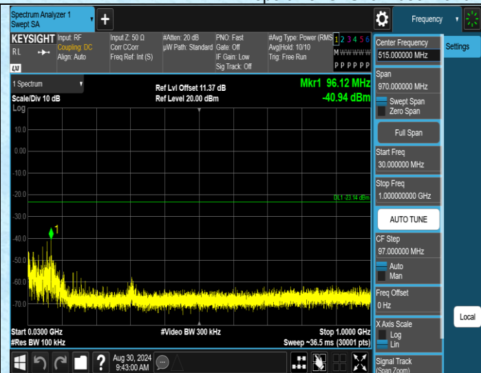
DH5-Ant1-2480-30-1000-PASS
