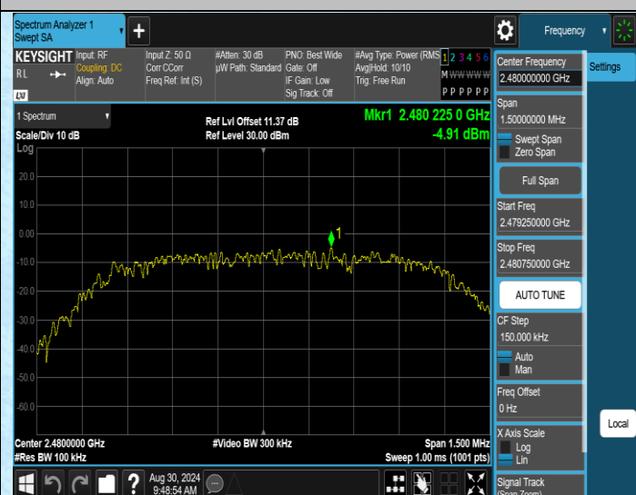
2DH5-Ant1-2480-0~Reference-PASS
