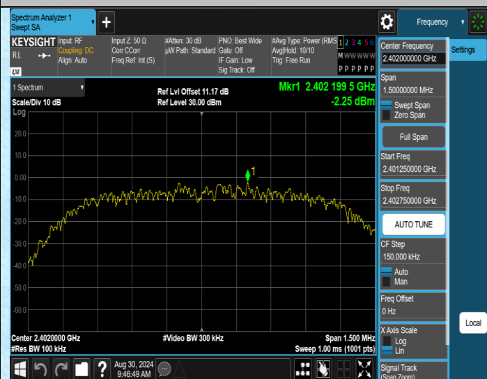
2DH5-Ant1-2402-0-Reference-PASS
