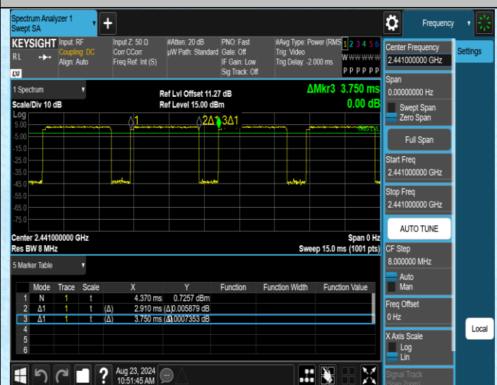
NTVN-3DH5-Ant1-2441
