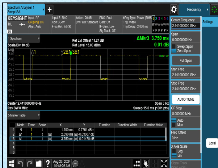
NTVN-2DH5-Ant1-2441
