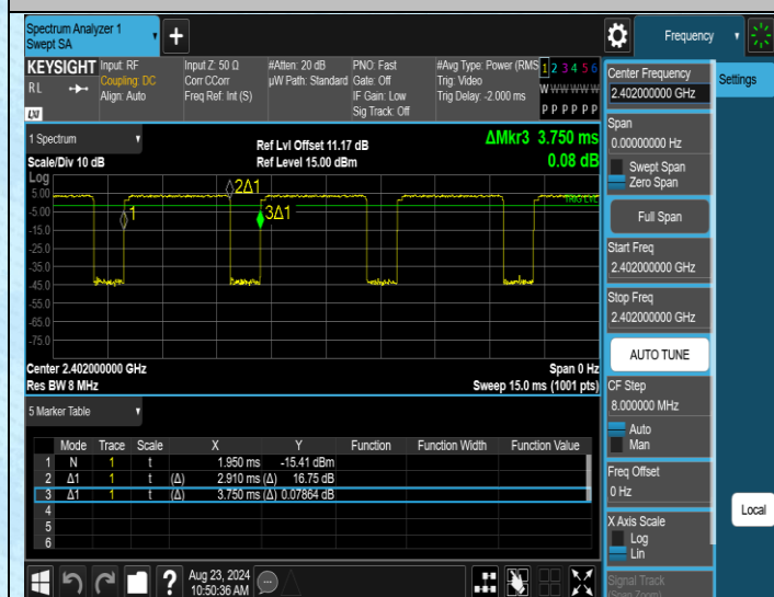
NTVN-3DH5-Ant1-2402
