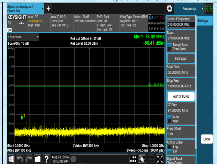
3DH5-Ant1-2480-30~1000-PASS
