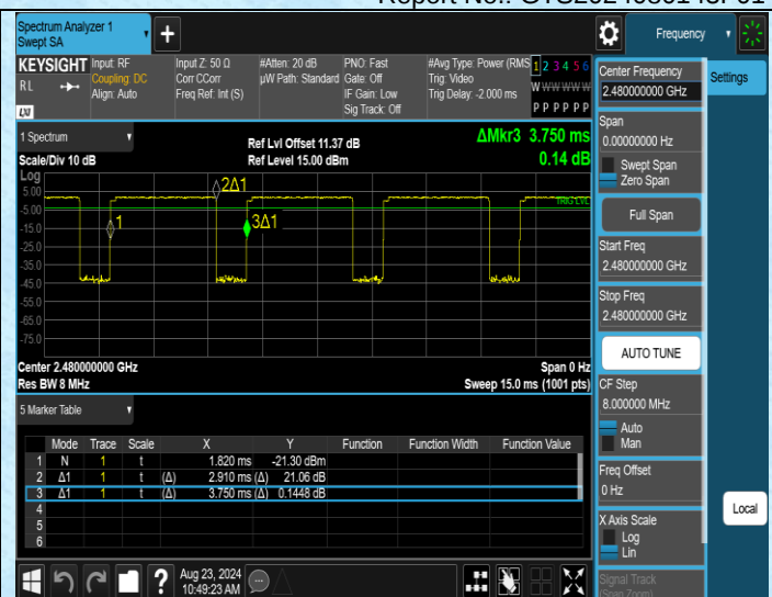
NTVN-2DH5-Ant1-2480
