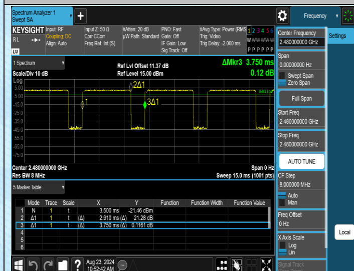
NTVN-3DH5-Ant1-2480
