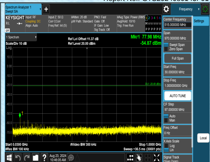
DH5-Ant1-2480-30~1000-PASS
