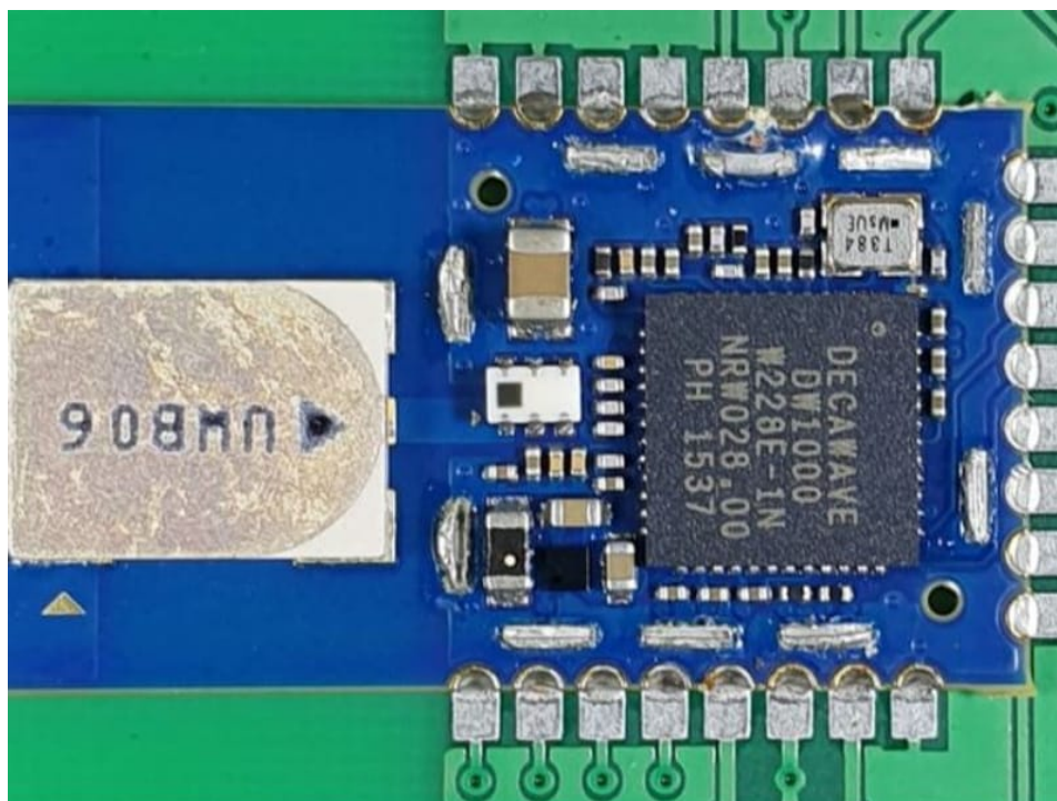
Photo 4: UWB chip, same model
