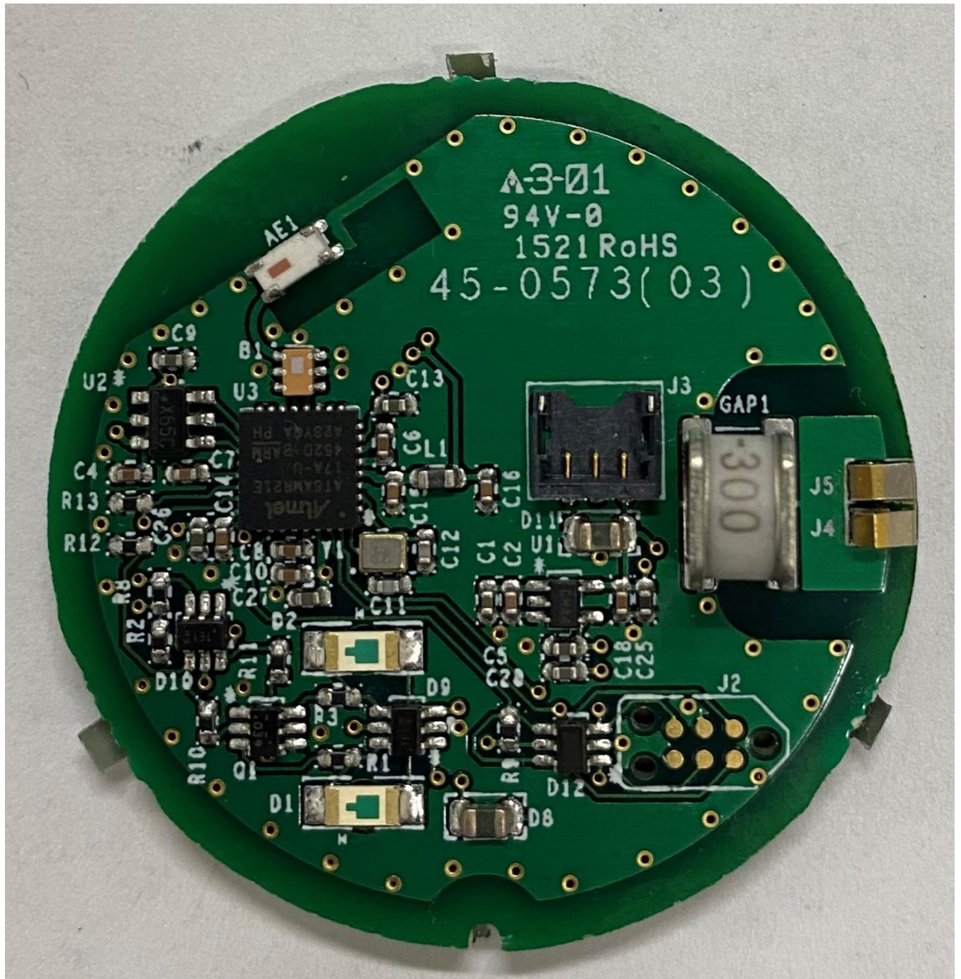
Component Placement
