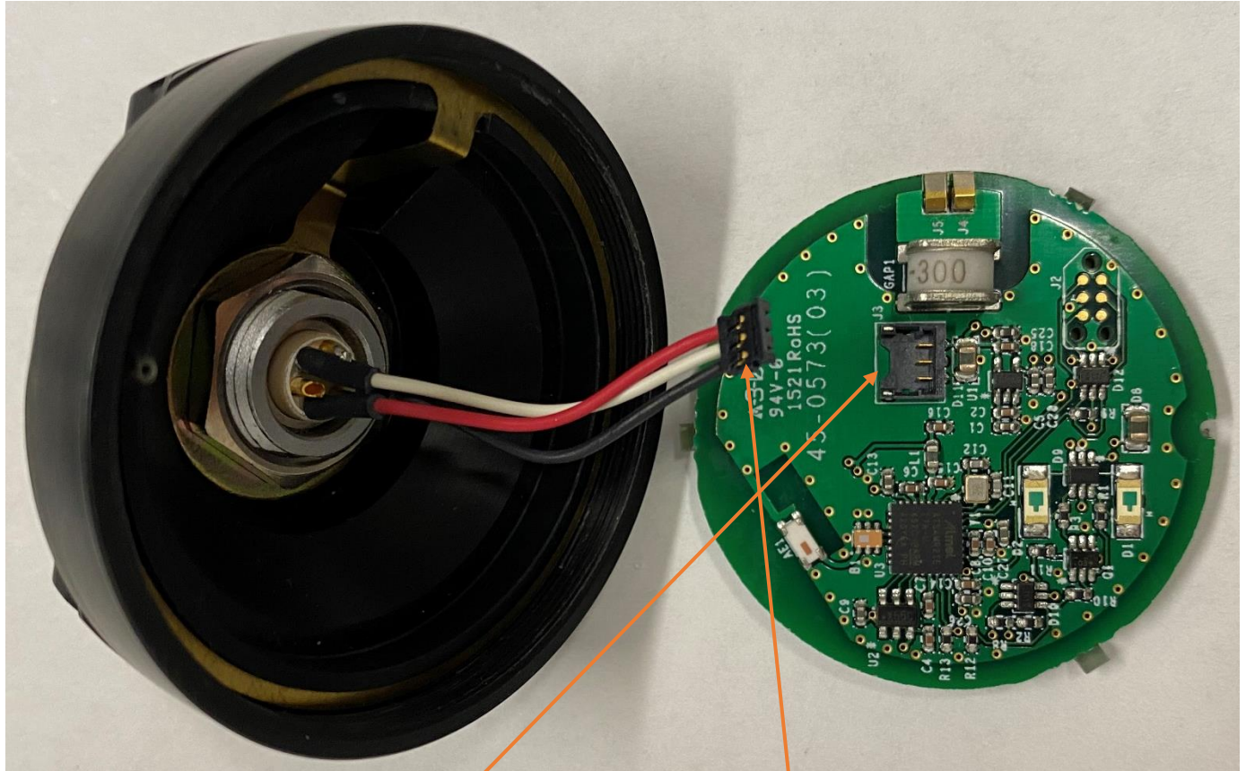
Molex header J3 connects to the Connector cable
