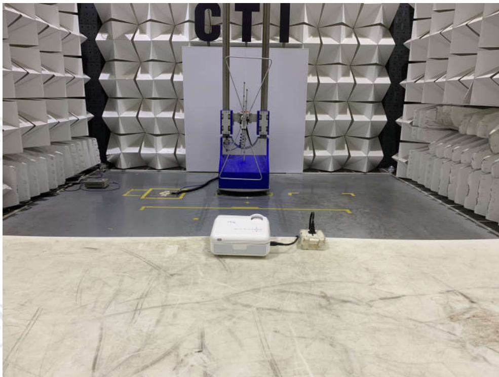
Radiated spurious emission Test Setup-1(Below 1GHz)
