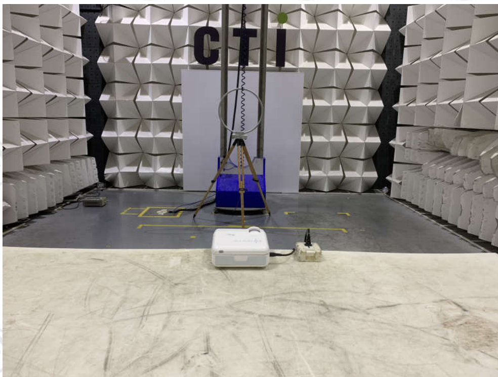
Radiated spurious emission Test Setup-3(Below 30MHz)
