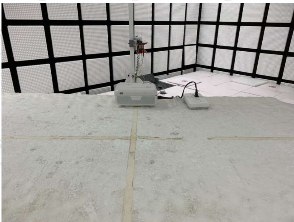
Radiated spurious emission Test Setup-2(Above 1GHz)
