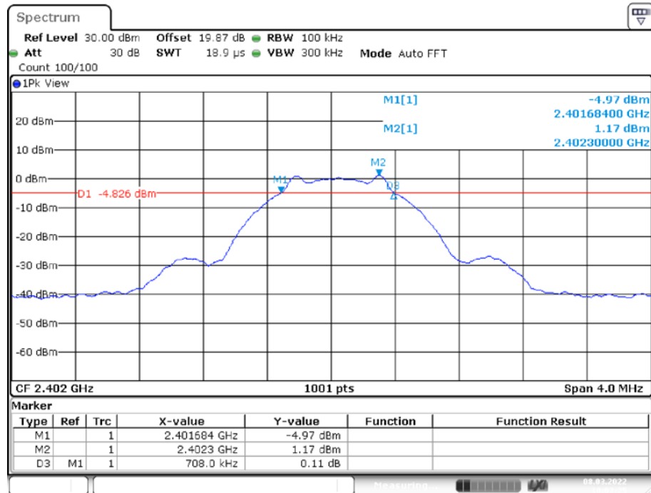
BLE_1M_Ant1_2402
