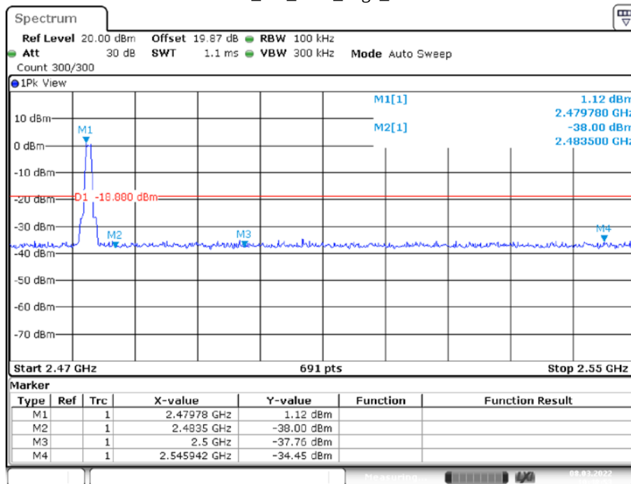
BLE_1M_Ant1_High_2480
