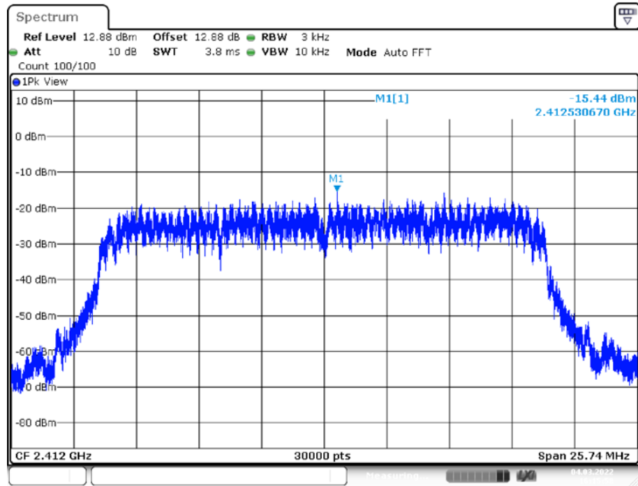
11N20SISO_Ant1_2412
