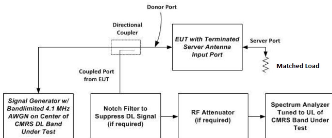
Test setup for uplink noise power measurement in the presence of a downlink signal
