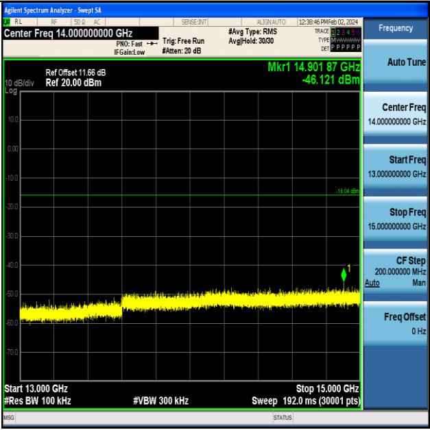
11B-Ant1-2412-13000~15000-PASS
