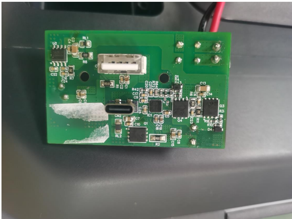
USB output module PCB view
