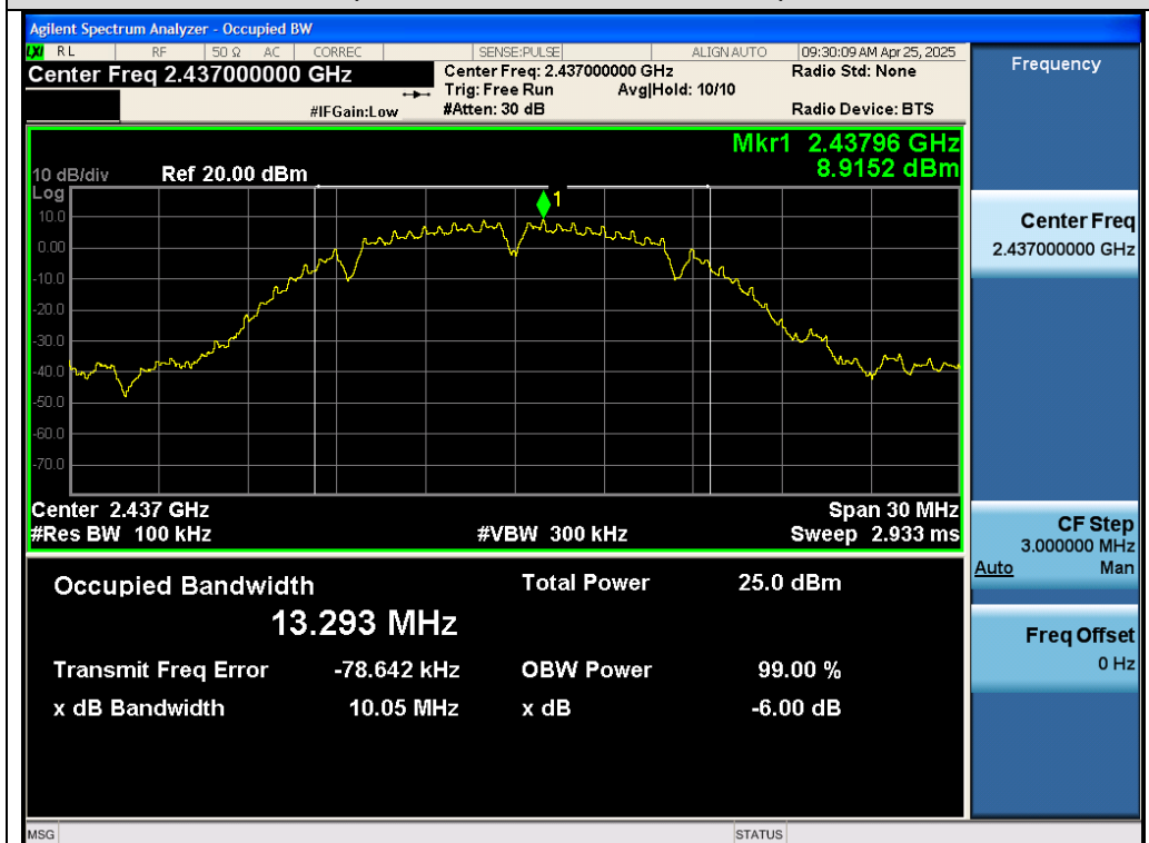
Test_Graph_802.11b_ANT1_2437_1Mbps_DTSSBW
