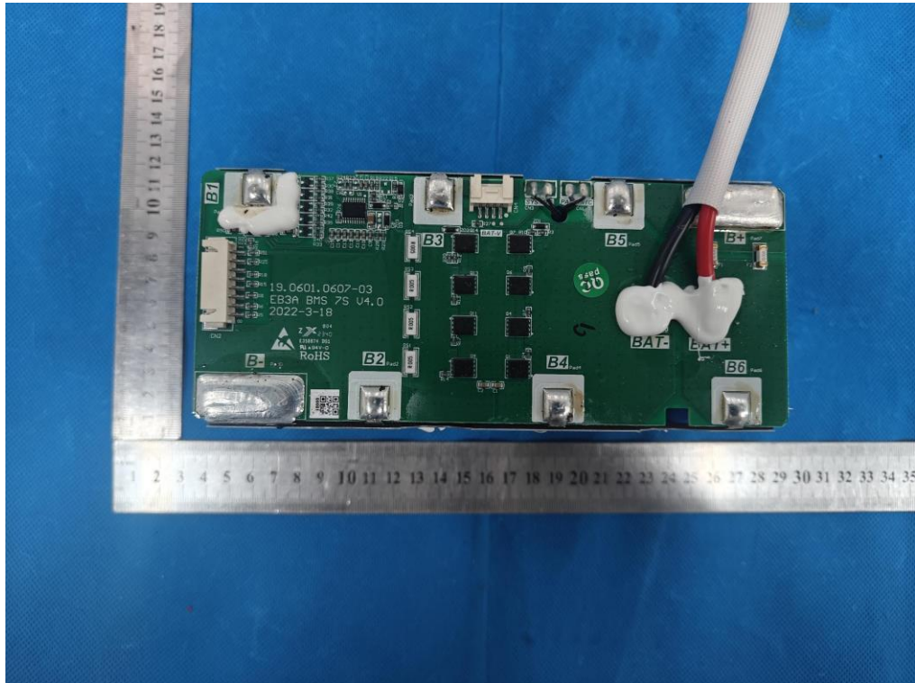
INTERNAL VIEW OF EUT (FIGURE 19)
