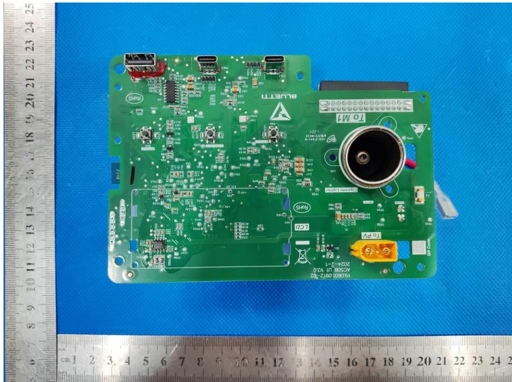
INTERNAL VIEW OF EUT (FIGURE 11)
