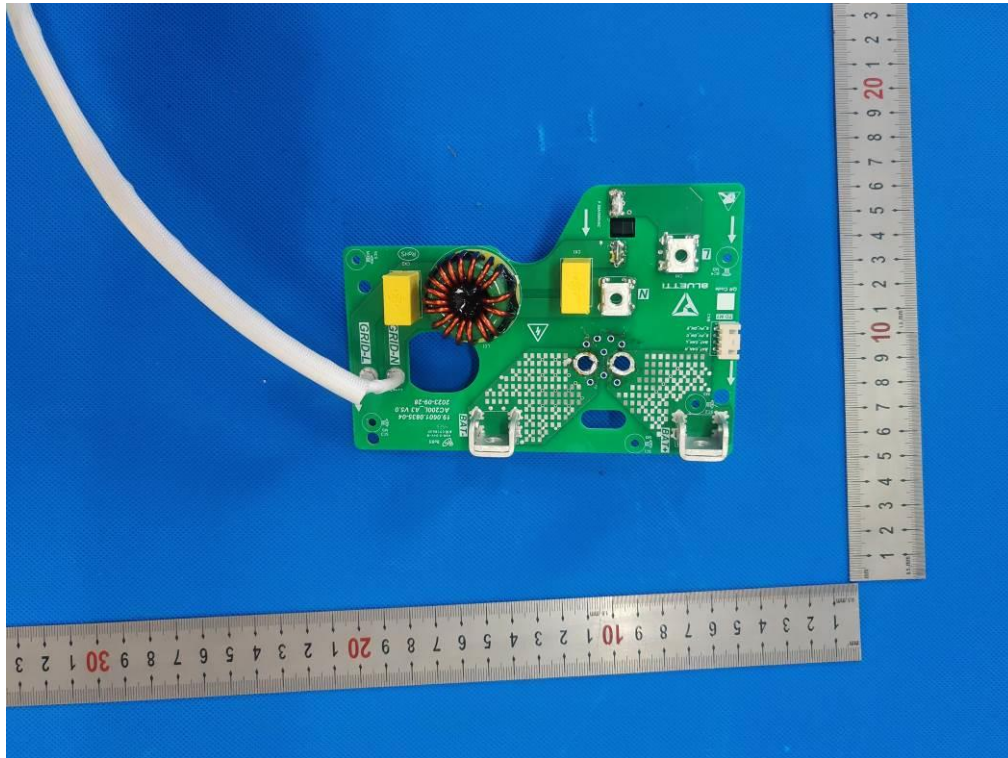
INTERNAL VIEW OF EUT (FIGURE 23)
