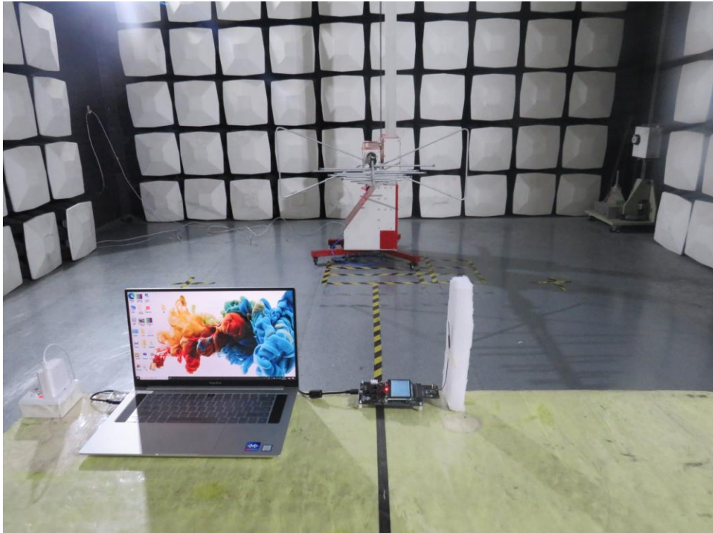
Radiated emission (Above 1GHz) -Antenna RF915-2
