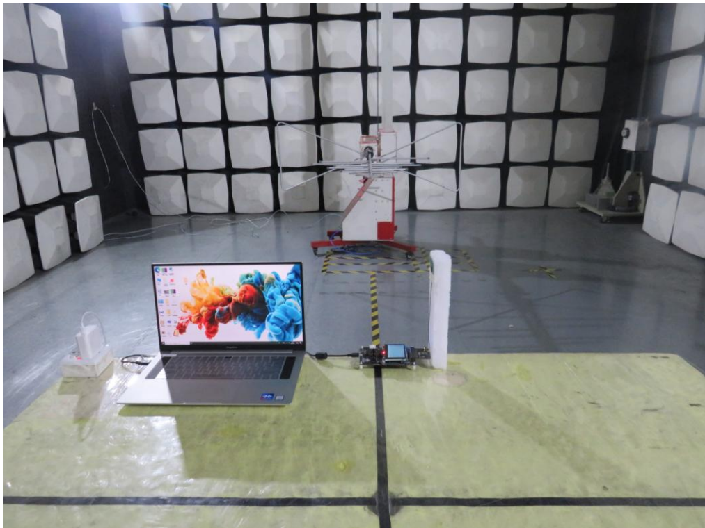
Radiated emission (30-1000MHz) -Antenna RF915-1
