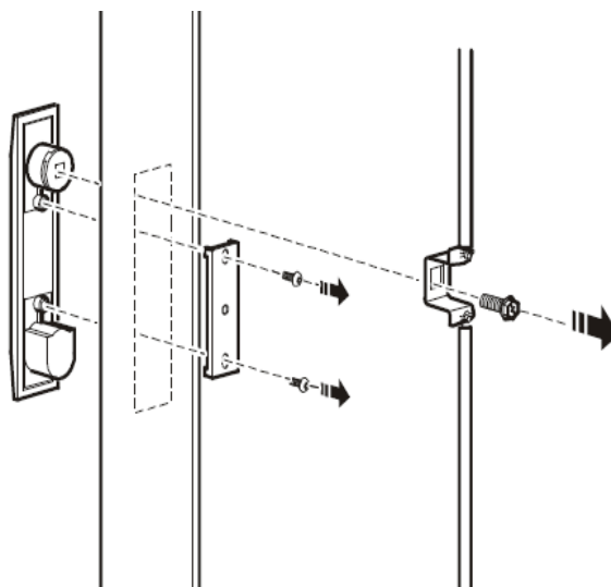
Typical door
