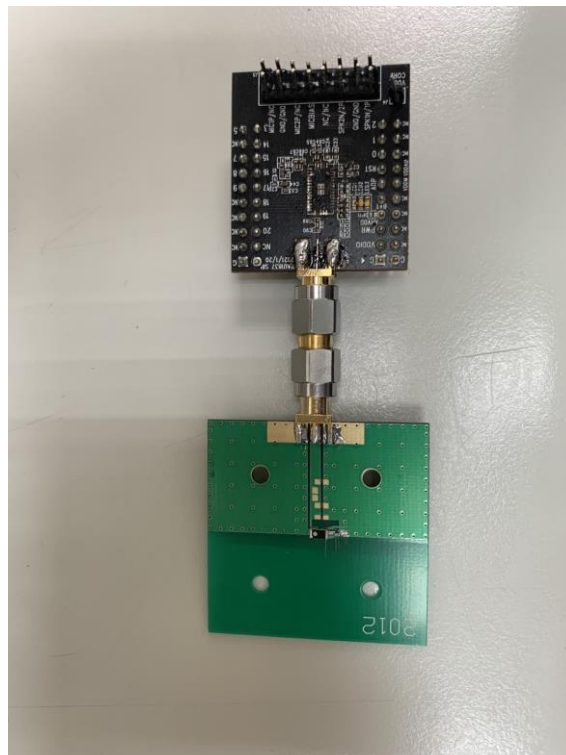
Antenna + Test Kit
