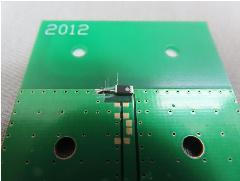
Antenna + Test Kit
