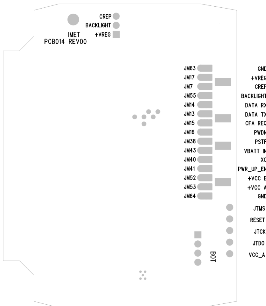
Figure 1 – Pin Layout
