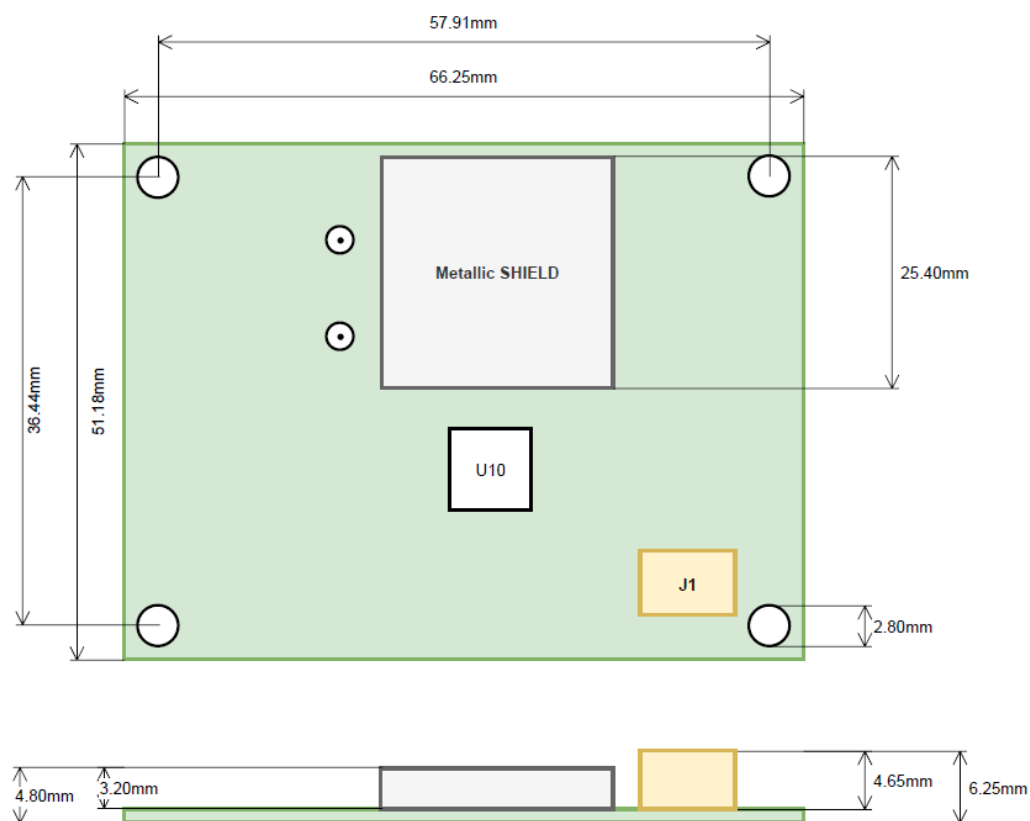
Figure 3 – Dimension Details
