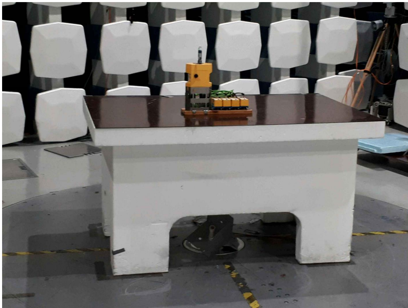
Measurement setup below 1000 MHz
