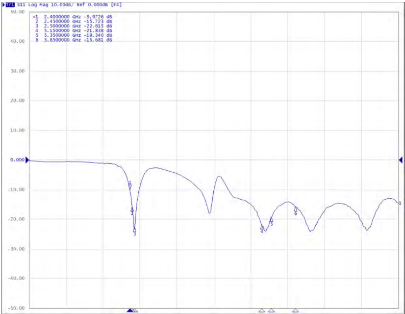
Figure 2 Return Loss
