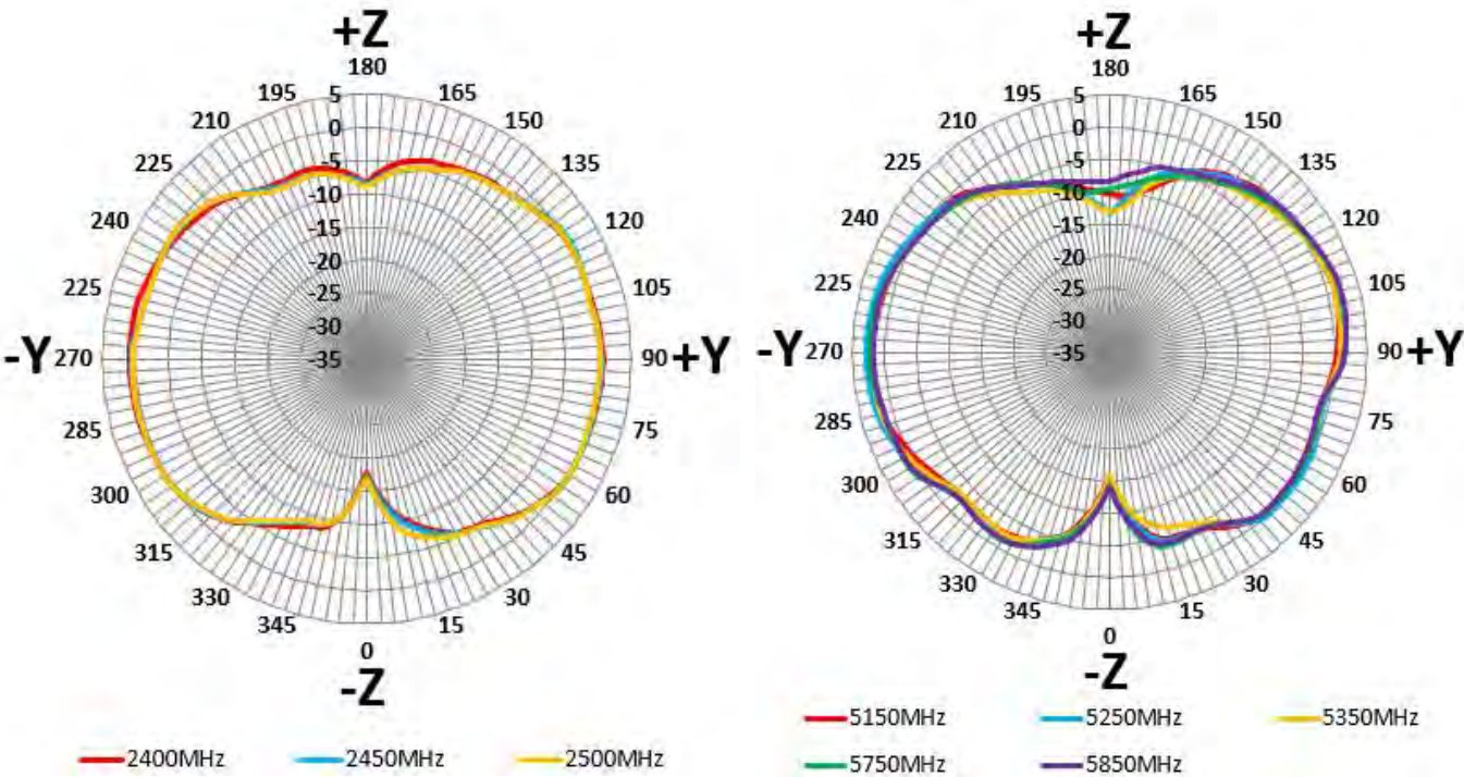
(C). Elevation 2 plane (YZ plane) radiation pattern
