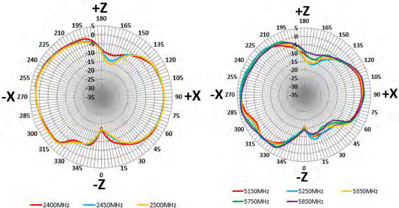
(B). Elevation 1 plane (XZ plane) radiation pattern
