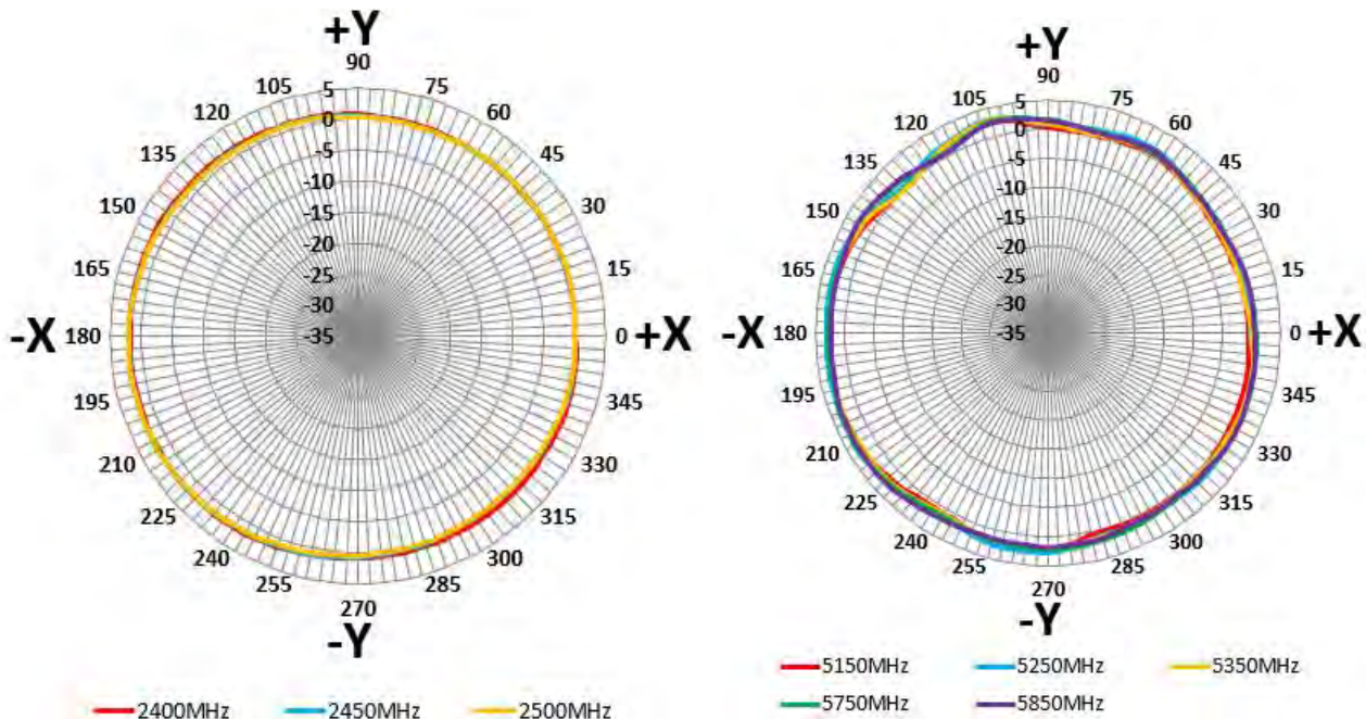
(A). Azimuth plane (XY plane) radiation pattern
