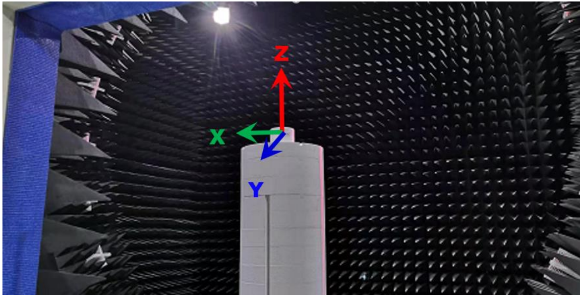
Figure 1 Measurement Orientation
