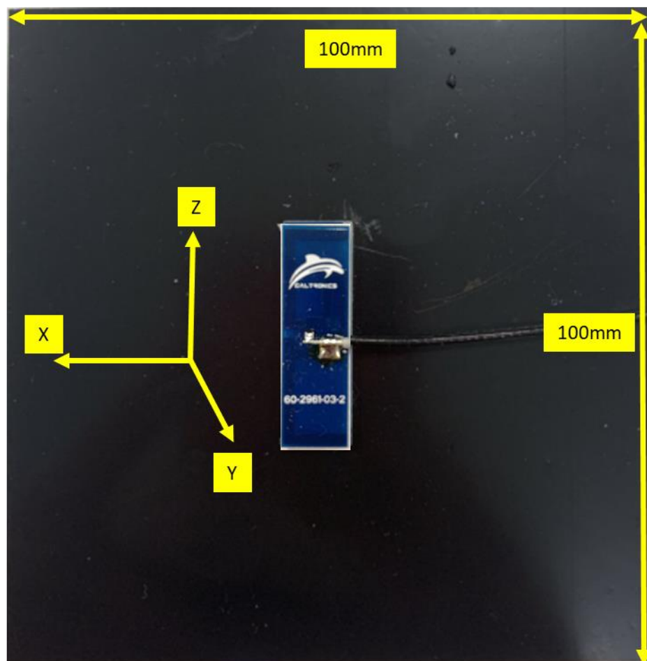
Figure 3 Measurement Orientation
